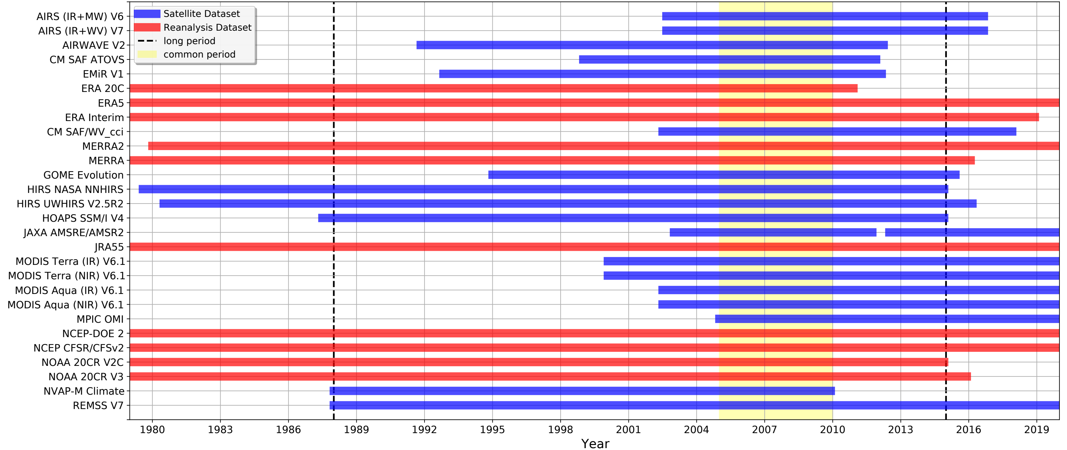
Ensemble members and time coverage from Version 2 of the G-VAP TCWV archive.
