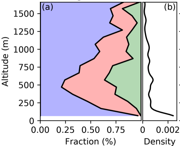
Open Ocean
