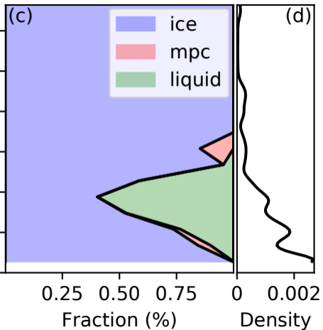
Sea Ice
