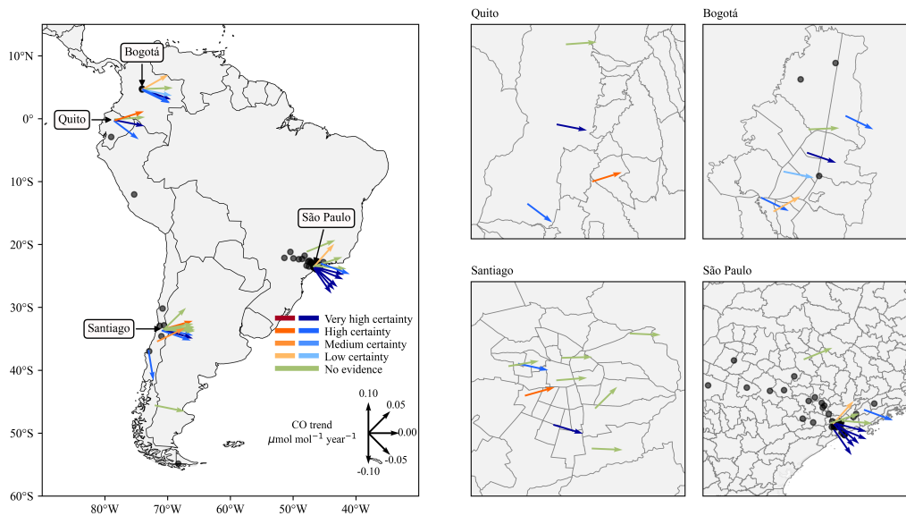
Figure S1: Ground-level carbon monoxide trends in \mu\text{mol mol}^{-1} \text{year}^{-1} and reliability levels calculated from available South American monitoring stations (left panel). When one or more change points are identified, the trend starts from the latest change point detected. The right panels focus on Bogotá, Quito, Santiago and São Paulo. The grey dots denote stations with no carbon monoxide monitoring or that did not meet data quality criteria.
