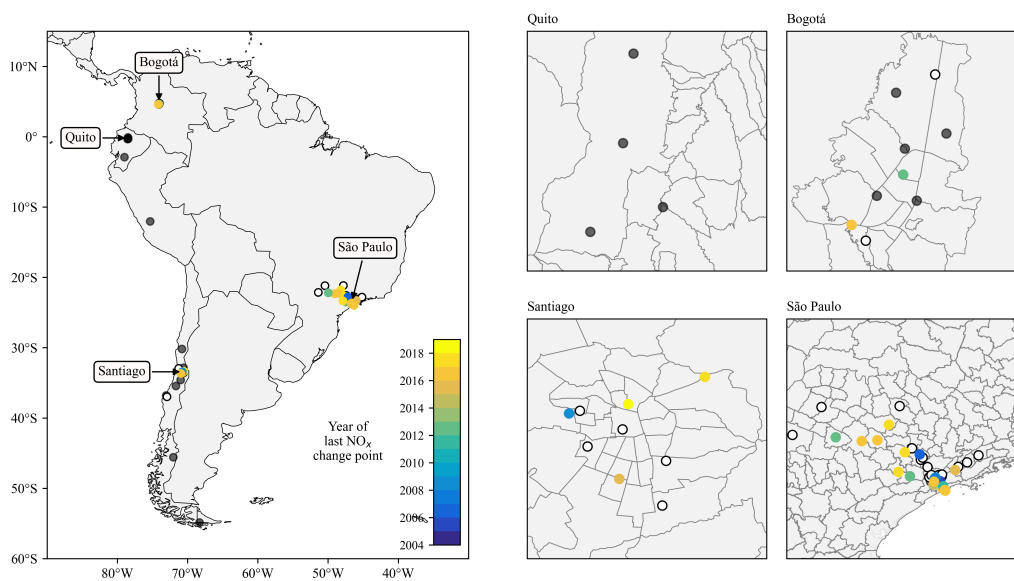
Figure S8: Year of the last detected \text{NO}_x trend change point in South American monitoring stations (left panel). The right panels focus on Bogotá, Quito, Santiago and São Paulo. The grey dots denote stations with no change point detected or that did not meet data quality criteria and the white dots denote stations with no trend change point detected.
