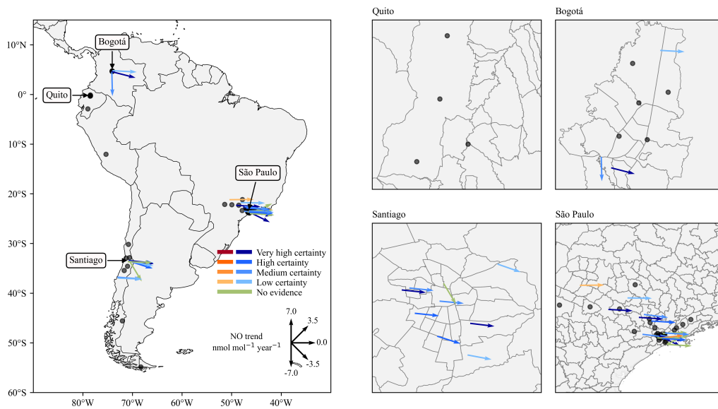
Figure S3: Ground-level nitric oxide trends in \text{nmol mol}^{-1} \text{ year}^{-1} and reliability levels calculated from available South American monitoring stations (left panel). When one or more change points are identified, the trend starts from the latest change point detected. The right panels focus on Bogotá, Quito, Santiago and São Paulo. The grey dots denote stations with no nitric oxide monitoring or that did not meet data quality criteria.
