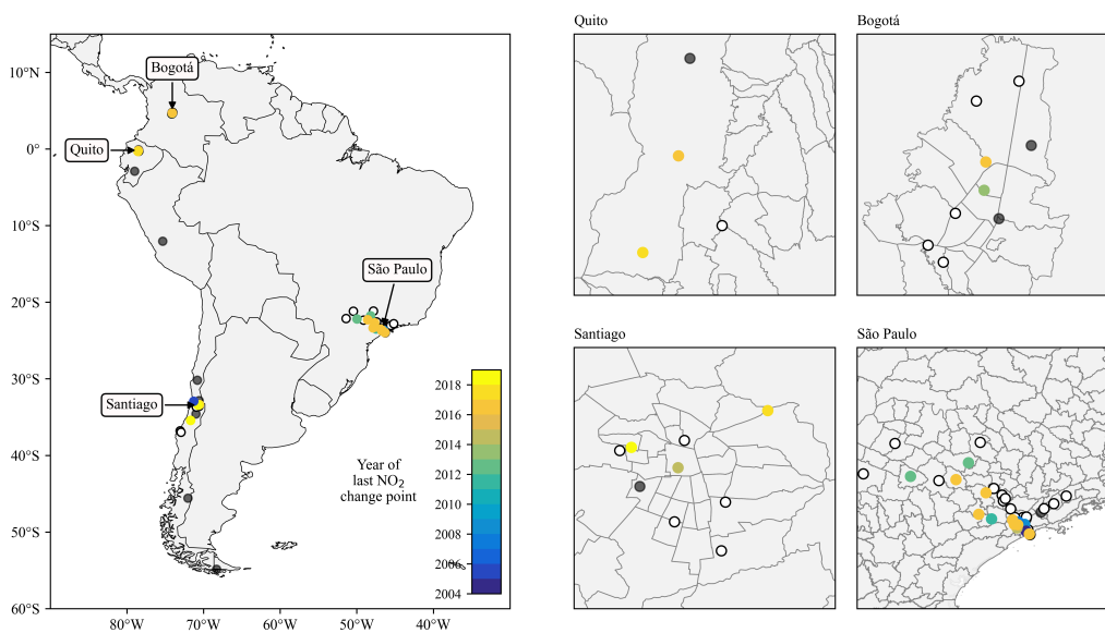
Figure S6: Year of the last detected nitrogen dioxide trend change point in South American monitoring stations (left panel). The right panels focus on Bogotá, Quito, Santiago and São Paulo. The grey dots denote stations with no change point detected or that did not meet data quality criteria and the white dots denote stations with no trend change point detected.
