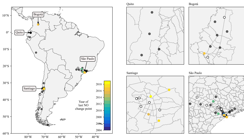
Figure S4: Year of the last detected nitric oxide trend change point in South American monitoring stations (left panel). The right panels focus on Bogotá, Quito, Santiago and São Paulo. The grey dots denote stations with no change point detected or that did not meet data quality criteria and the white dots denote stations with no trend change point detected.
