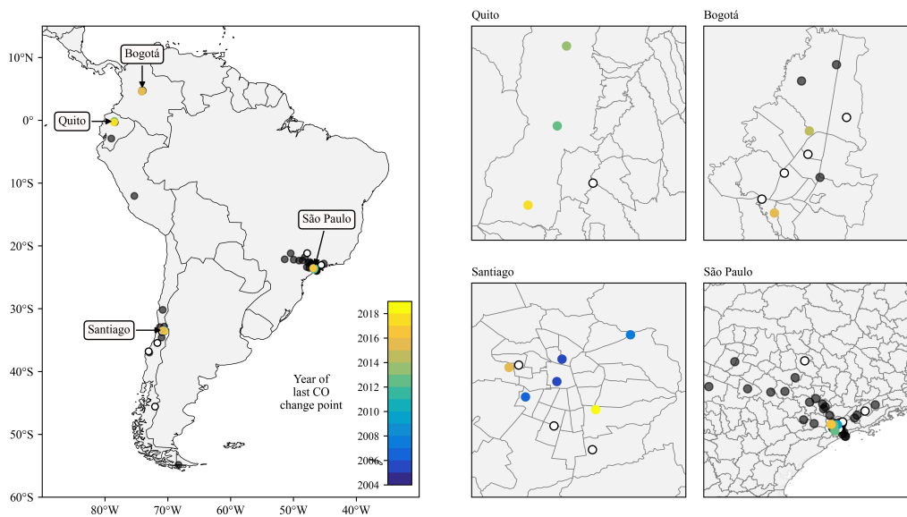
Figure S2: Year of the last detected carbon monoxide trend change point in South American monitoring stations (left panel). The right panels focus on Bogotá, Quito, Santiago and São Paulo. The grey dots denote stations with no carbon monoxide monitoring or that did not meet data quality criteria and the white dots denote stations with no trend change point detected.
