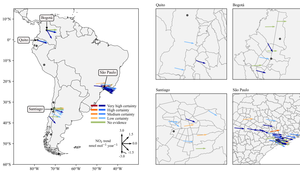
Figure S5: Ground-level nitrogen dioxide trends in \text{nmol mol}^{-1} \text{ year}^{-1} and reliability levels calculated from available South American monitoring stations (left panel). When one or more change points are identified, the trend starts from the latest change point detected. The right panels focus on Bogotá, Quito, Santiago and São Paulo. The grey dots denote stations with no nitrogen dioxide monitoring or that did not meet data quality criteria.
