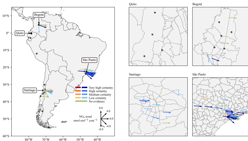
Figure S7: Ground-level \text{NO}_x trends in \text{nmol mol}^{-1} \text{ year}^{-1} and reliability levels calculated from available South American monitoring stations (left panel). When one or more change points are identified, the trend starts from the latest change point detected. The right panels focus on Bogotá, Quito, Santiago and São Paulo. The grey dots denote stations with no nitrogen oxides monitoring or that did not meet data quality criteria.
