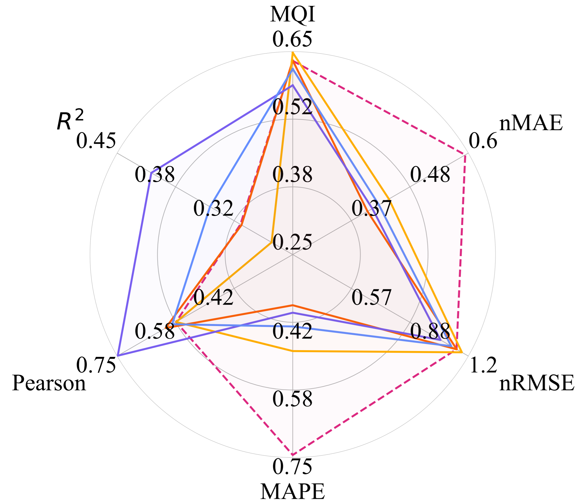
Urban Background - NOx
