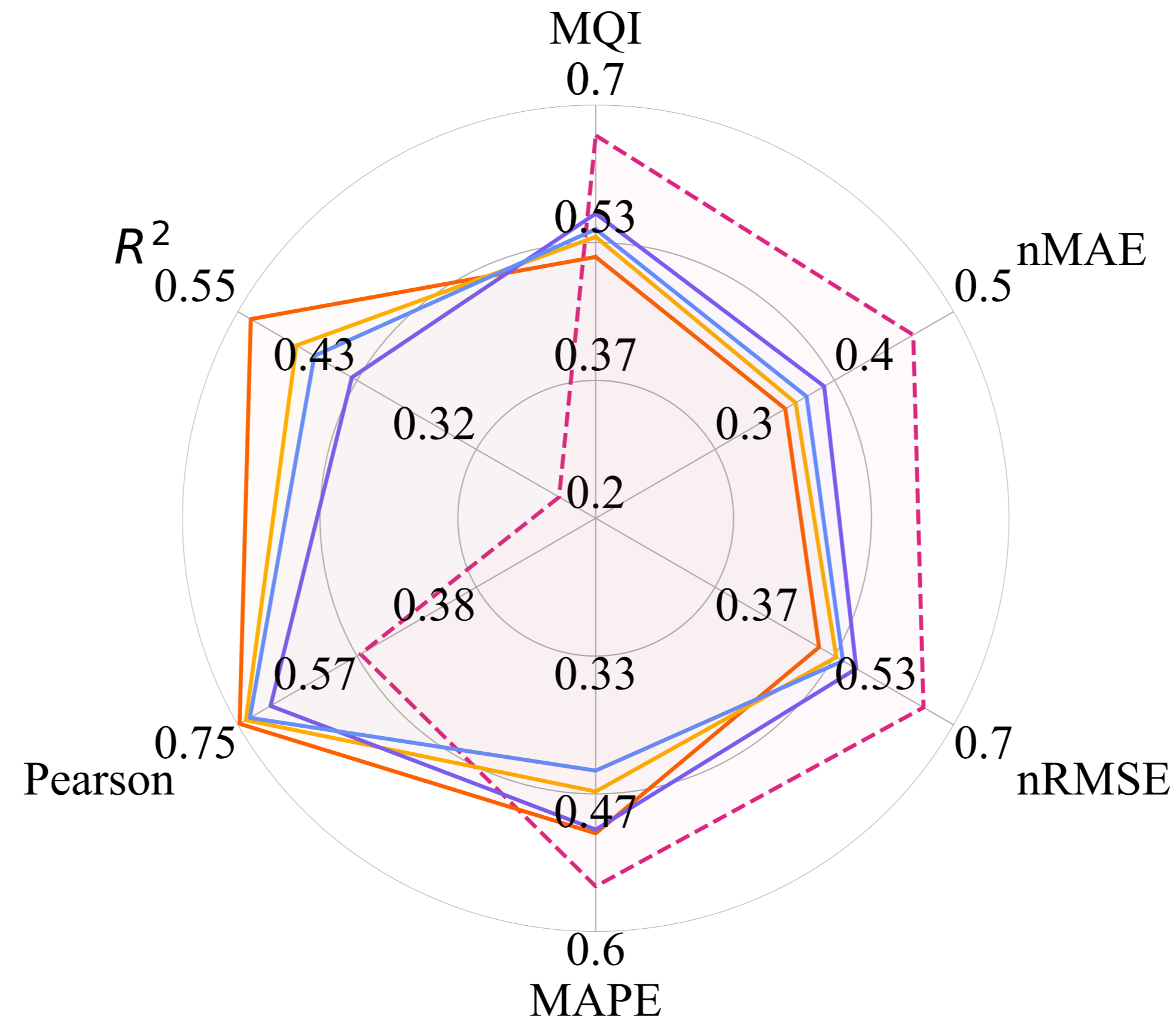
Urban Background - PM10
