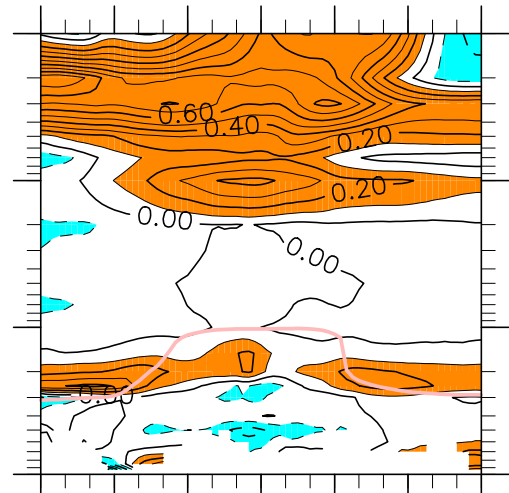
(b) JRA-55 - REM
