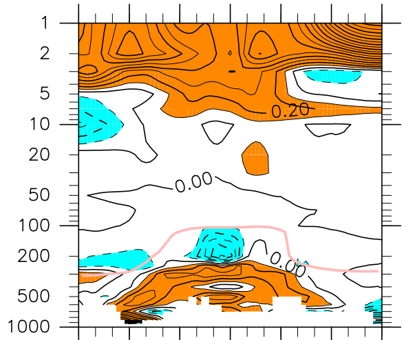
(a) MERRA-2 - REM
