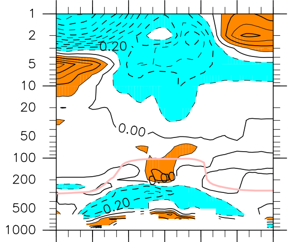
(c) ERA-Int - REM
