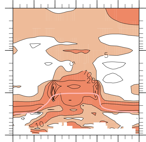
(f) (SD / |REM|) x 100%
