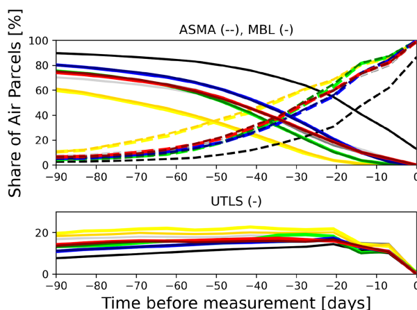
(b) Vertical Classification
