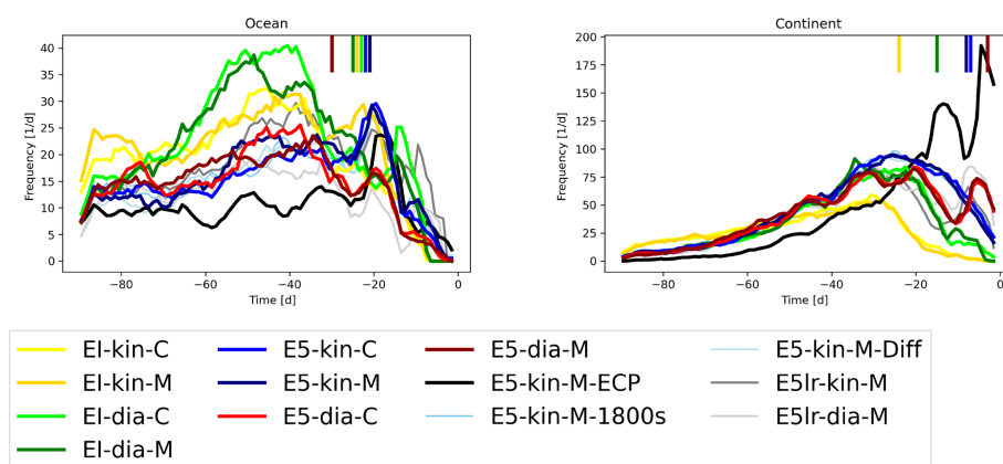
(a) Horizontal Classification
