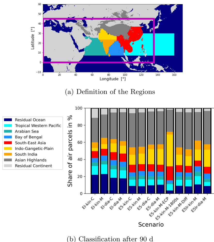
Figure 3. Panel (a) shows the definition of contributing regions. The purple box marks an area that contains most of the air parcels that circulate in the ASMA. Panel (b) shows the horizontal classification of the air parcels according to the surface regions after a 90 d backward trajectory time. Shown is the fraction of air parcels that reach the MBL.
