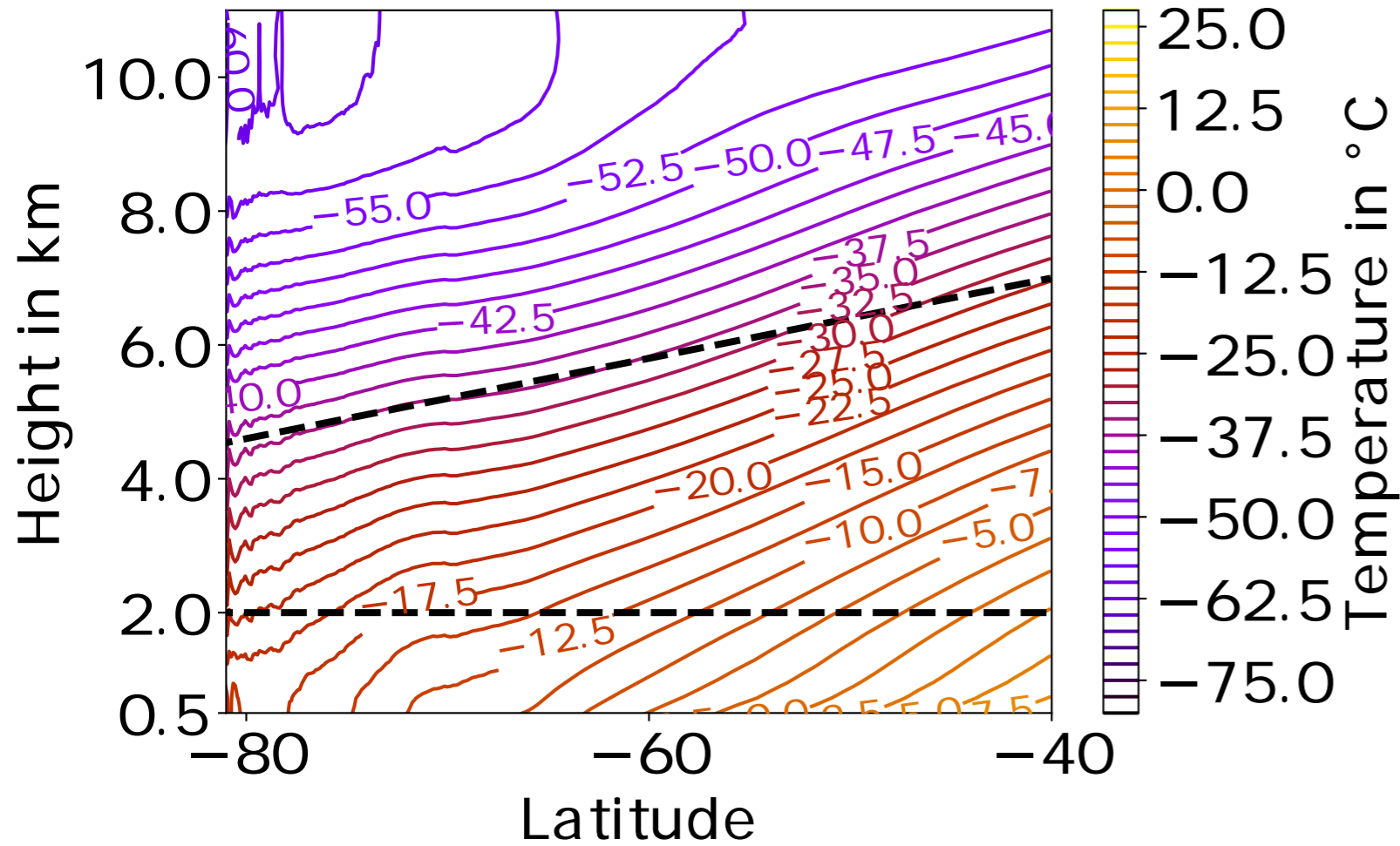
(a) Southern Ocean
