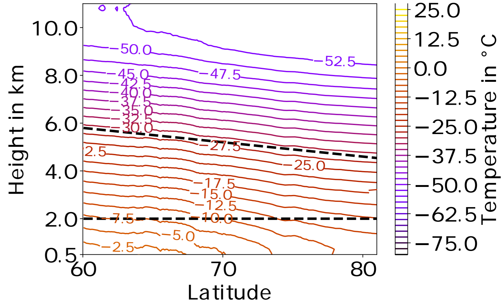
(b) Arctic marine regions
