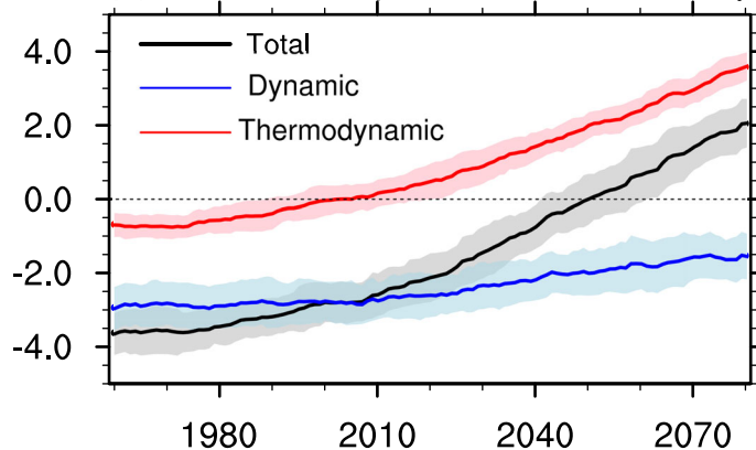
(c) SAT anomaly °C
