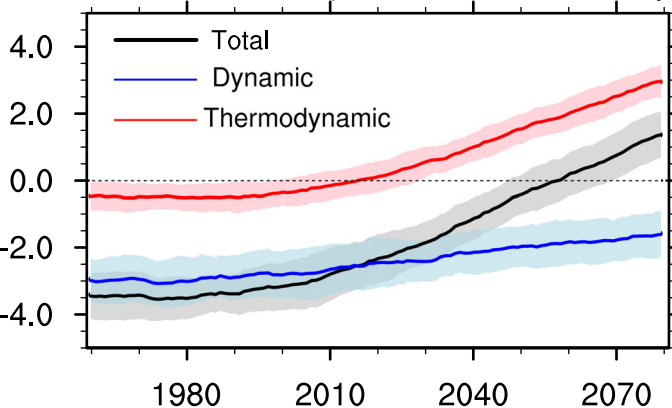
(a) SAT anomaly °C
