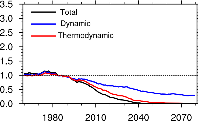
(b) Occurrence probability ratio SAT
