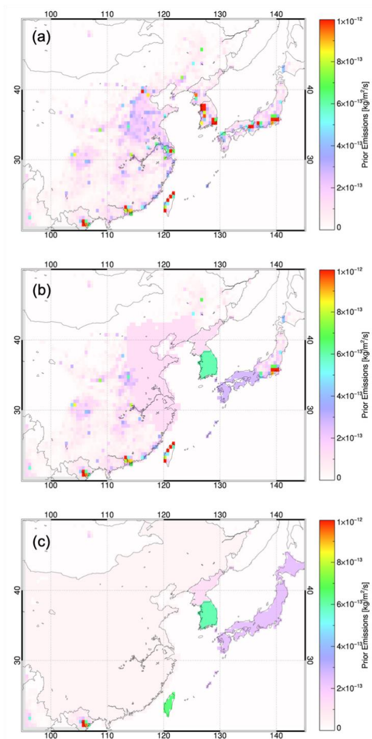
20 Figure S1: Types for the prior emission distribution used in FLEXPART-FLEXINVERT+, (a) population distribution, (b) eastern Asia flatten, and (c) Asia flatten, respectively. For each HFC substance, the prior spatial distribution of each type is the same, the only difference is magnitude of each pixel.
