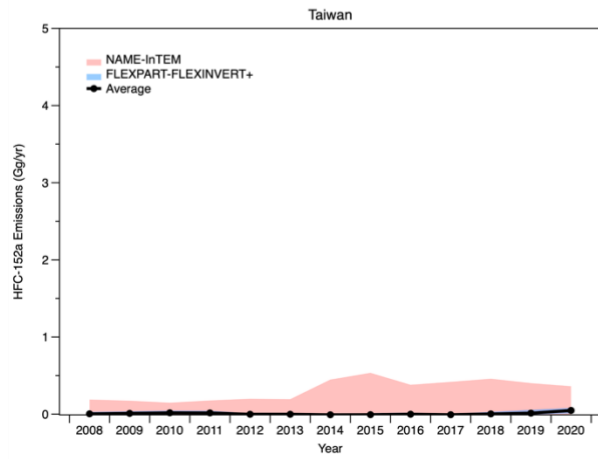
Figure S6: Same as Fig. S2, but for HFC-152a.
