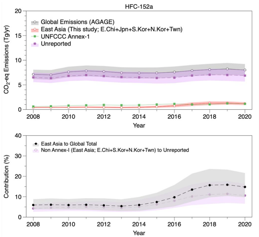
70 Figure S13: Same as Fig. S10, but for HFC-152a.
