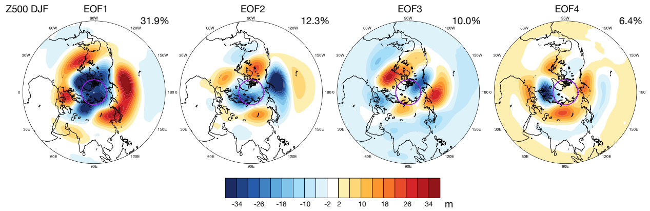
Figure S3: The first 4 EOF patterns of northern hemisphere Z500 (0°-90°N). Spatial variance explained by each EOF is shown on the top-right corner of each panel. Unit in m.
