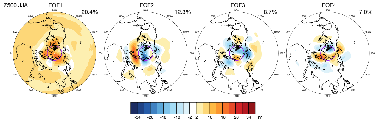
Figure S9: Similar to Fig. S3, but for summer.
