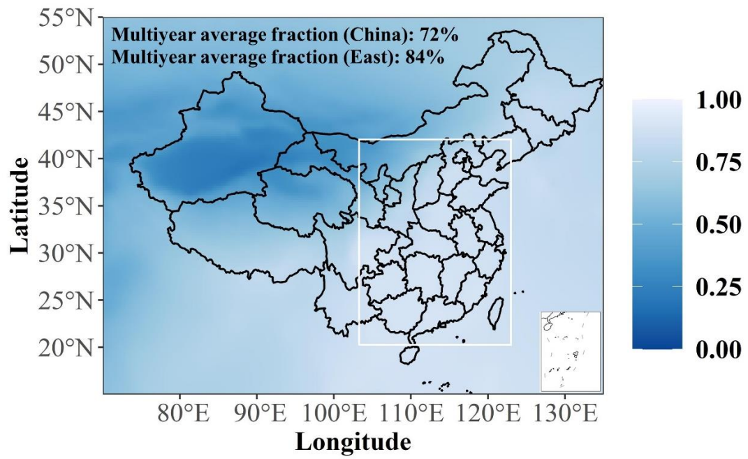
Figure S11 Multiyear average fractions of BC AAOD to AAOD from MERRA-2.
