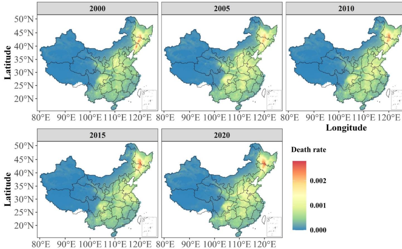
Figure S9 Spatial distribution of premature mortality rate attributable to the posterior BC exposure during 2000-2020 (with a five-year interval).
