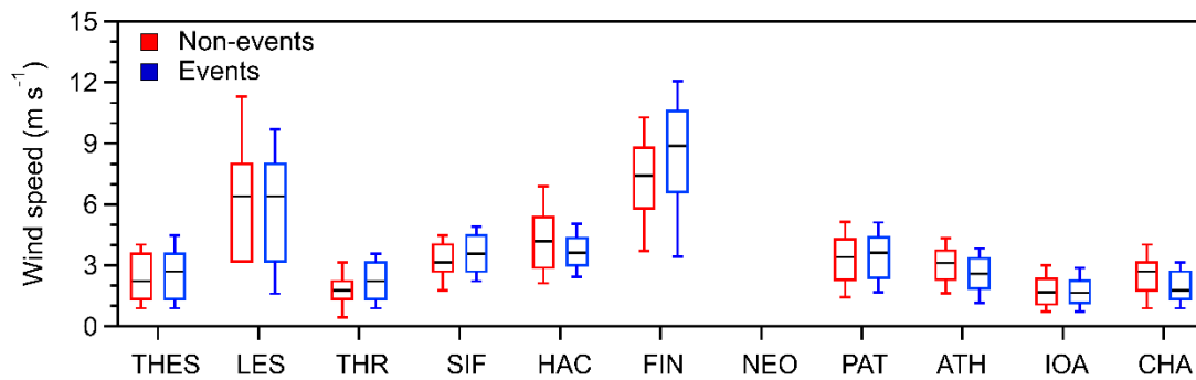
Figure S4: Comparison of the average wind speed in the period between 8:00 and 18:00 LT during nucleation events and non-events in each station. The black lines represent the median, while the box edges the 25 th and 75 th percentiles. The whiskers correspond to the 10 th and 90 th percentiles.
