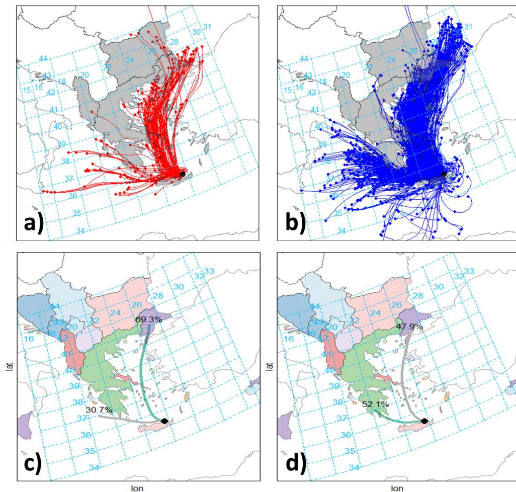
Figure S11: The 24-h backward air trajectories arriving at Finokalia during both campaigns in 2020 and 2021 for: a) NPF (Class I and II) events (178 trajectories); b) the whole period (1362 trajectories). The probabilities of the air masses originating from a specific location during c) NPF events and d) the whole period is also shown. The trajectories shown for the NPF events correspond only to the hours during which the particles appeared during each event. The trajectories for the rest of the days correspond to the hours between 7:00–19:00 LT. Maps created by R version 4.1.1 using the Openair (Carslaw and Ropkins, 2012) version 2.16-0 and the MapData 2022 packages.
