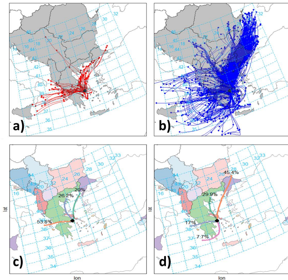
Figure S14: The 24-h backward air trajectories arriving at Athens during both campaigns in 2020 and 2021 for: a) NPF (Class I and II) events (73 trajectories); b) the whole period (1307 trajectories). The probabilities of the air masses originating from a specific location during c) NPF events and d) the whole period is also shown. The trajectories shown for the NPF events correspond only to the hours during which the particles appeared during each event. The trajectories for the rest of the days correspond to the hours between 7:00–19:00 LT. Maps created by R version 4.1.1 using the Openair (Carslaw and Ropkins, 2012) version 2.16-0 and the MapData 2022 packages.
