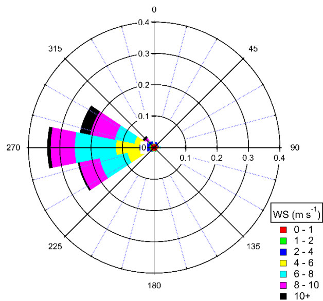
Figure S13: Local wind direction and speed during the summer campaign of 2020 in Finokalia.
