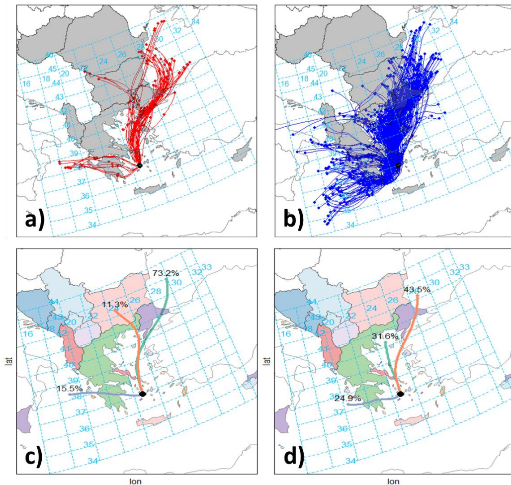
Figure S9: The 24-h backward air trajectories arriving at Sifnos during both campaigns in 2020 and 2021 for: a) NPF (Class I and II) events (134 trajectories); b) the whole period (880 trajectories). The probabilities of the air masses originating from a specific location during c) NPF events and d) the whole period is also shown. The trajectories shown for the NPF events correspond only to the hours during which the particles appeared during each event. The trajectories for the rest of the days correspond to the hours between 7:00–19:00 LT. Maps created by R version 4.1.1 using the Openair (Carslaw and Ropkins, 2012) version 2.16-0 and the MapData 2022 packages.
