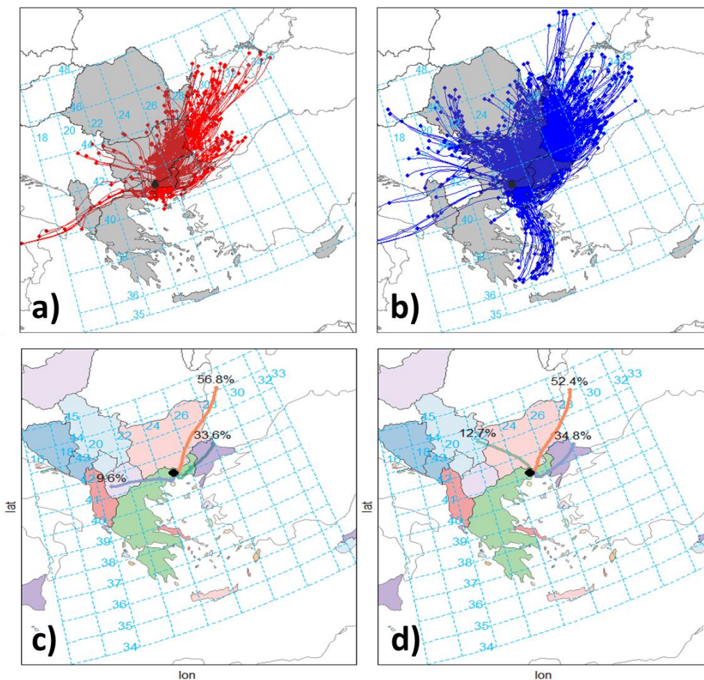
Figure S7: The 24-h backward air trajectories arriving at Thrace during both campaigns in 2020 and 2021 for: a) NPF (Class I and II) events (275 trajectories); b) the whole period (1227 trajectories). The probabilities of the air masses originating from a specific location during c) NPF events and d) the whole period is also shown. The trajectories shown for the NPF events correspond only to the hours during which the particles appeared during each event. The trajectories for the rest of the days correspond to the hours between 7:00–19:00 LT. Maps created by R version 4.1.1 using the Openair (Carslaw and Ropkins, 2012) version 2.16-0 and the MapData 2022 packages.
