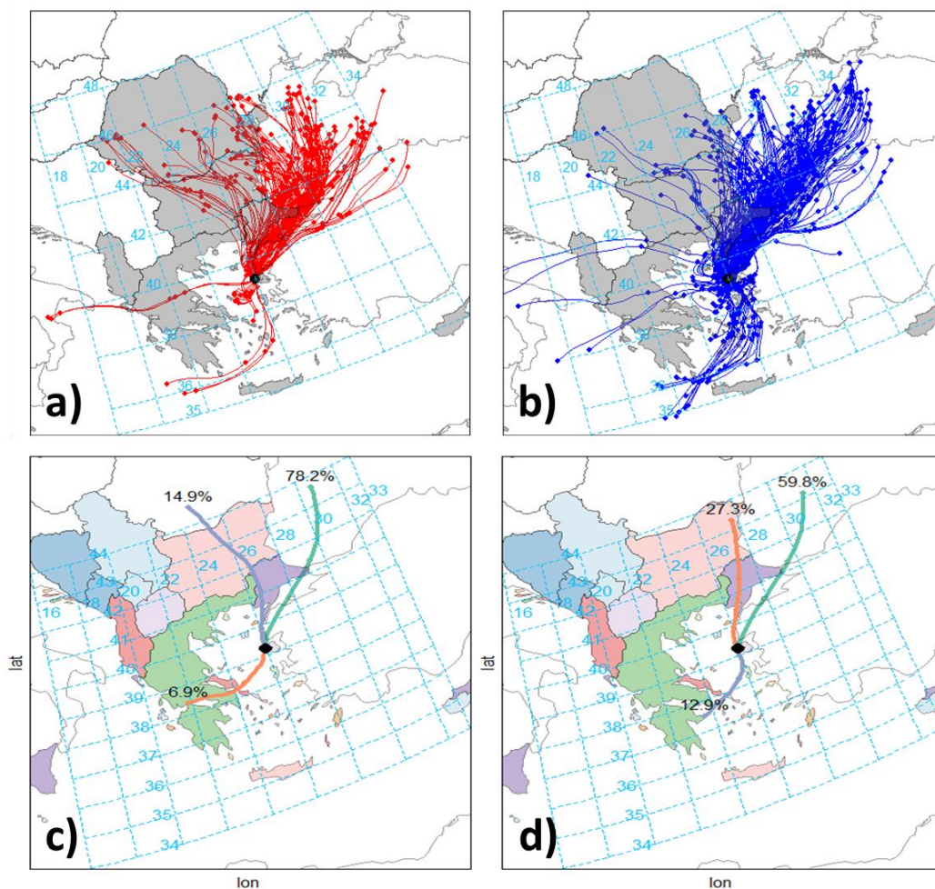
Figure S8: The 24-h backward air trajectories arriving at Lesvos during both campaigns in 2020 and 2021 for: a) NPF (Class I and II) events (197 trajectories); b) the whole period (543 trajectories). The probabilities of the air masses originating from a specific location during c) NPF events and d) the whole period is also shown. The trajectories shown for the NPF events correspond only to the hours during which the particles appeared during each event. The trajectories for the rest of the days correspond to the hours between 7:00–19:00 LT. Maps created by R version 4.1.1 using the Openair (Carslaw and Ropkins, 2012) version 2.16-0 and the MapData 2022 packages.
