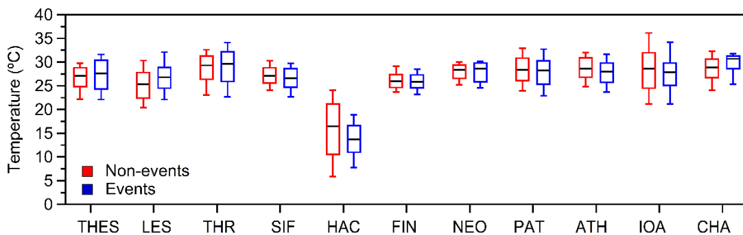
Figure S5: Comparison of the average temperature in the period between 8:00 and 18:00 LT during nucleation events and non-events in each station. The black lines represent the median, while the box edges the 25 th and 75 th percentiles. The whiskers correspond to the 10 th and 90 th percentiles.
