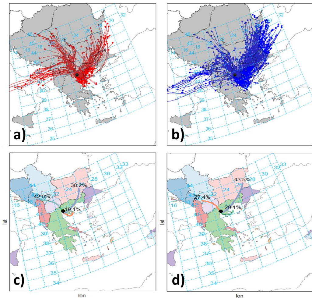
Figure S6: The 24-h backward air trajectories arriving at Thessaloniki during both campaigns in 2020 and 2021 for: a) NPF (Class I and II) events (257 trajectories); b) the whole period (877 trajectories). The probabilities of the air masses originating from a specific location during c) NPF events and d) the whole period is also shown. The trajectories shown for the NPF events correspond only to the hours during which the particles appeared during each event. The trajectories for the rest of the days correspond to the hours between 7:00–19:00 LT. Maps created by R version 4.1.1 using the Openair (Carslaw and Ropkins, 2012) version 2.16-0 and the MapData 2022 packages.
