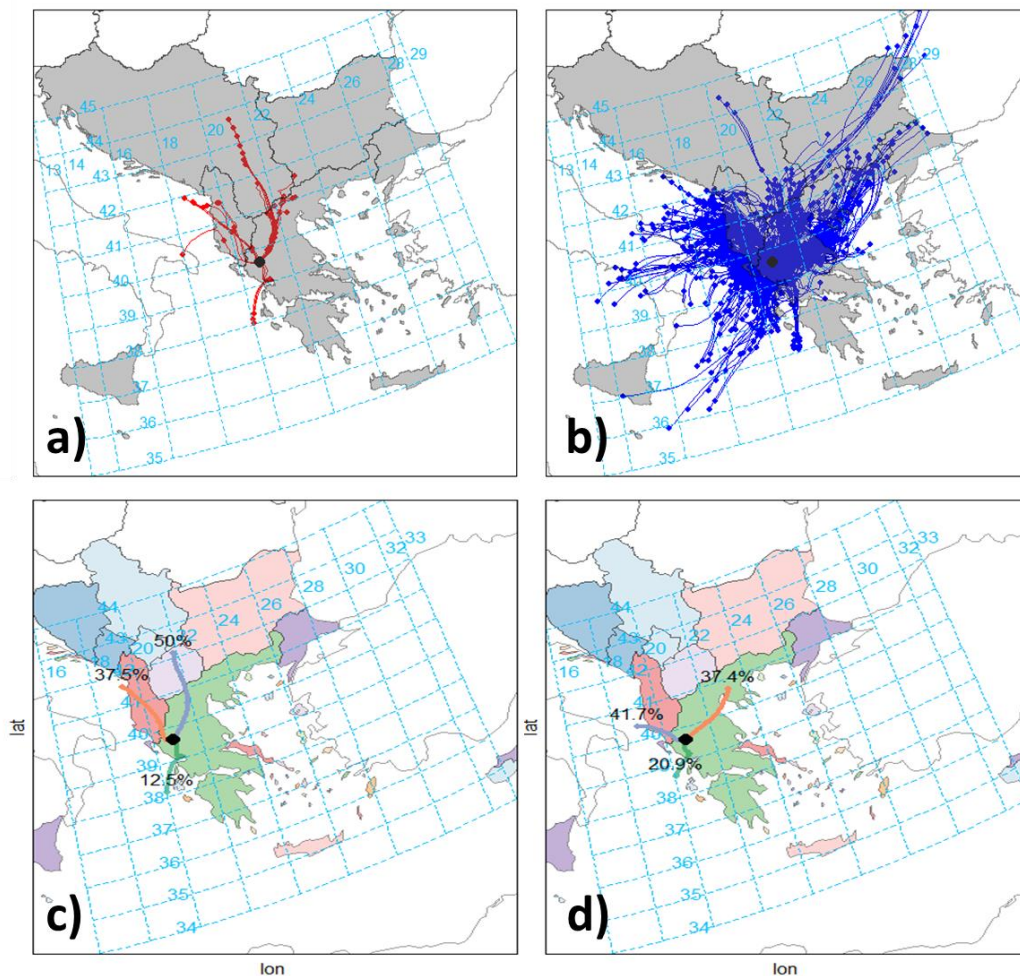
Figure S15: The 24-h backward air trajectories arriving at Ioannina during both campaigns in 2020 and 2021 for: a) NPF (Class I and II) events (26 trajectories); b) the whole period (809 trajectories). The probabilities of the air masses originating from a specific location during c) NPF events and d) the whole period is also shown. The trajectories shown for the NPF events correspond only to the hours during which the particles appeared during each event. The trajectories for the rest of the days correspond to the hours between 7:00–19:00 LT. Maps created by R version 4.1.1 using the Openair (Carslaw and Ropkins, 2012) version 2.16-0 and the MapData 2022 packages.
