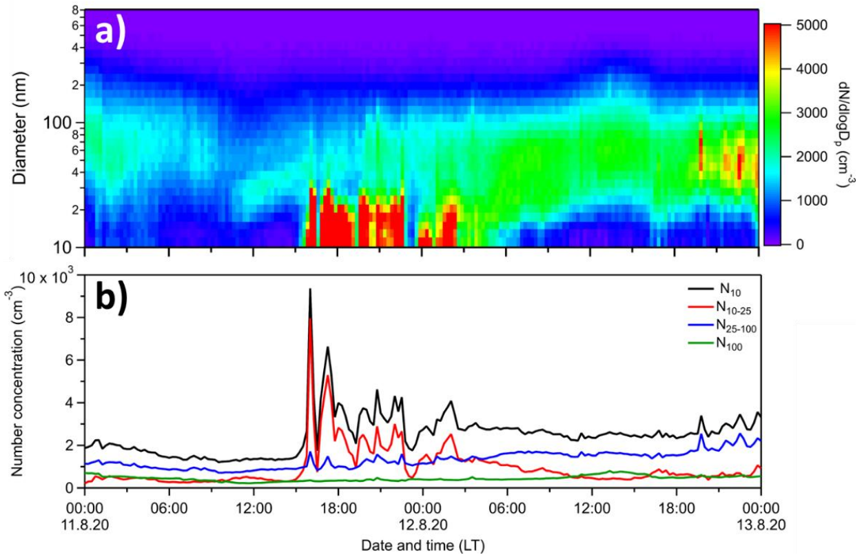
Figure S2: Example of a period where nighttime formation of new particles and subsequent growth was observed in NEO. The concentrations of the N_{10} , N_{10-25} , N_{25-100} and N_{100} are also shown.
