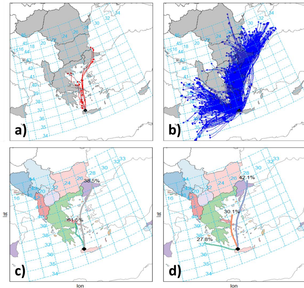
Figure S10: The 24-h backward air trajectories arriving at Chania during both campaigns in 2020 and 2021 for: a) NPF (Class I and II) events (13 trajectories); b) the whole period (1056 trajectories). The probabilities of the air masses originating from a specific location during c) NPF events and d) the whole period is also shown. The trajectories shown for the NPF events correspond only to the hours during which the particles appeared during each event. The trajectories for the rest of the days correspond to the hours between 7:00–19:00 LT. Maps created by R version 4.1.1 using the Openair (Carslaw and Ropkins, 2012) version 2.16-0 and the MapData 2022 packages.
