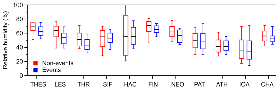
Figure S3: Comparison of the average relative humidity (RH) in the period between 8:00 and 18:00 LT during nucleation events and non-events in each station. The black lines represent the median, while the box edges the 25th and 75th percentiles. The whiskers correspond to the 10th and 90th percentiles.
