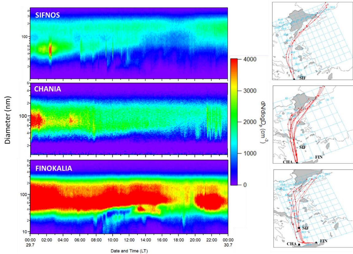
Figure S12: Particle number size distributions and the corresponding air mass trajectories (during the hours of the NPF event in Finokalia) in a) Sifnos, b) Chania and c) Finokalia. Maps created by R version 4.1.1 using the Openair (Carslaw and Ropkins, 2012) version 2.16-0 and the MapData 2022 packages.
