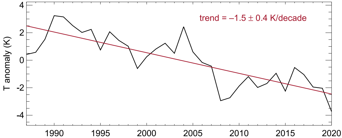
(b) Stratospheric temperature
