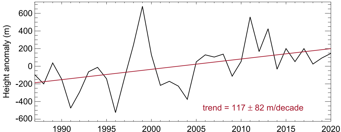
(c) Tropopause height
