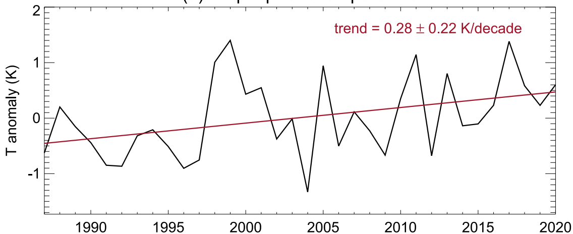
(a) Tropospheric temperature
