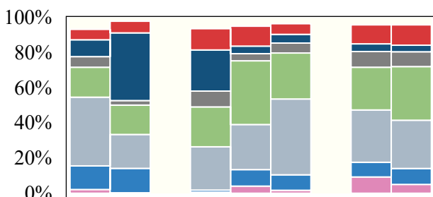
(e) WSOC-CHONS group
