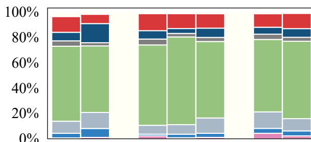
(b) WSOC-CHO group
