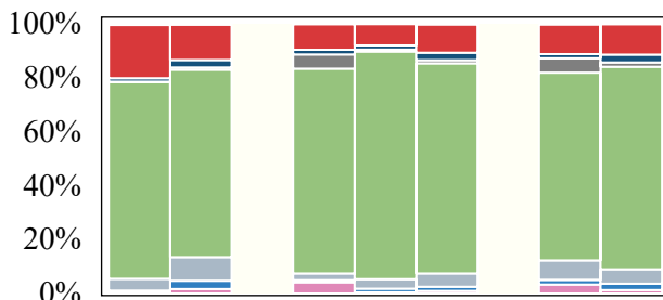
(c) WSOC-CHON group
