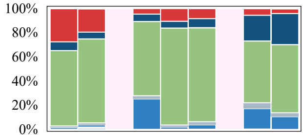
(h) WIOC-CHON group
