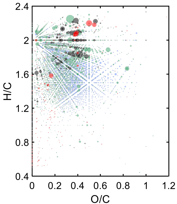
gas flaring + wildfire (N07)
