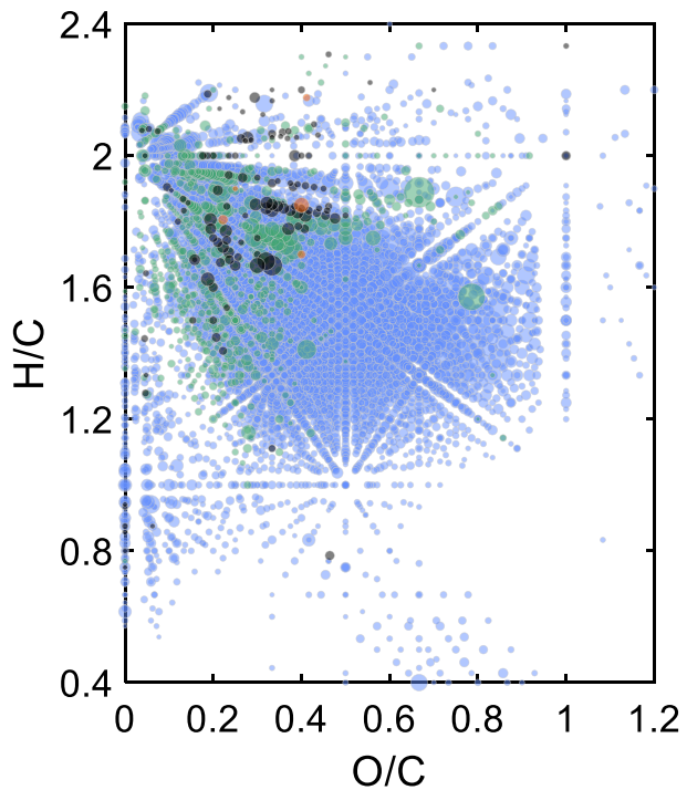
Bely Island (B01)
