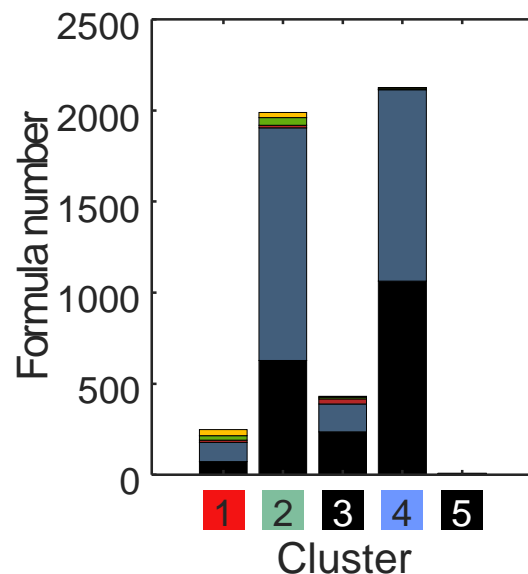
gas flaring + wildfire (N07)
