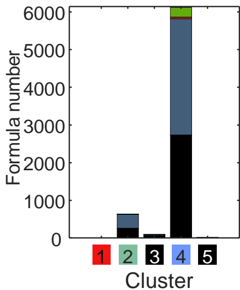
Bely Island (B01)
