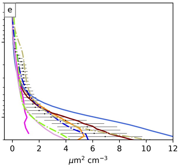
SAD Laramie (41°N, 105°W)
