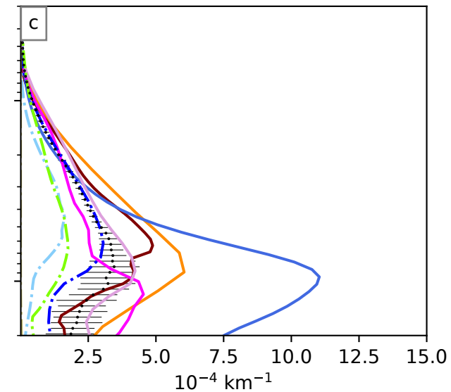
Extinction at 0.5 \mu\text{m} (30°S - 30°N)
