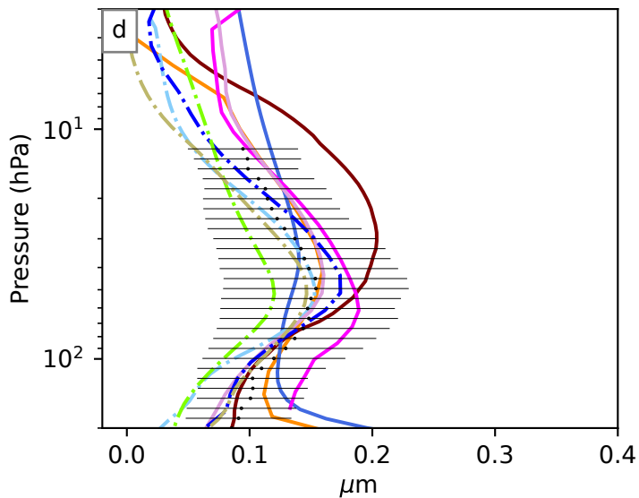
Effective radius Laramie (41°N, 105°W)
