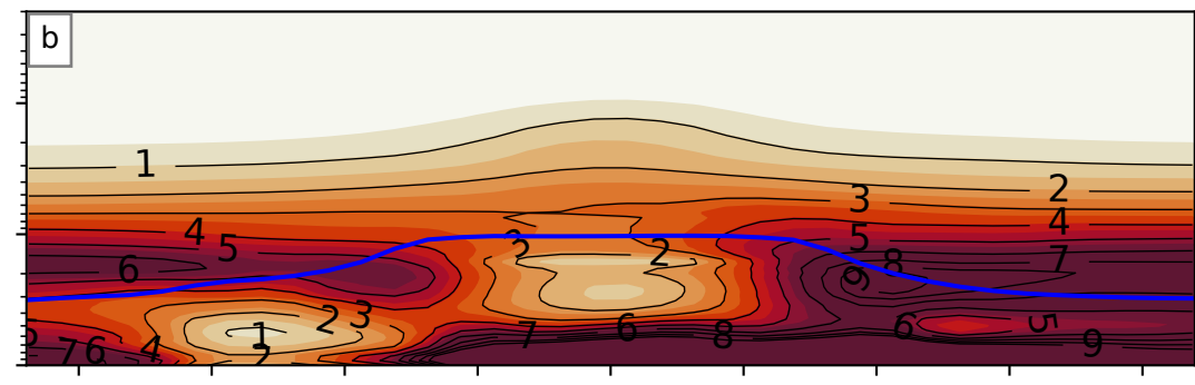
ECHAM5-HAM
