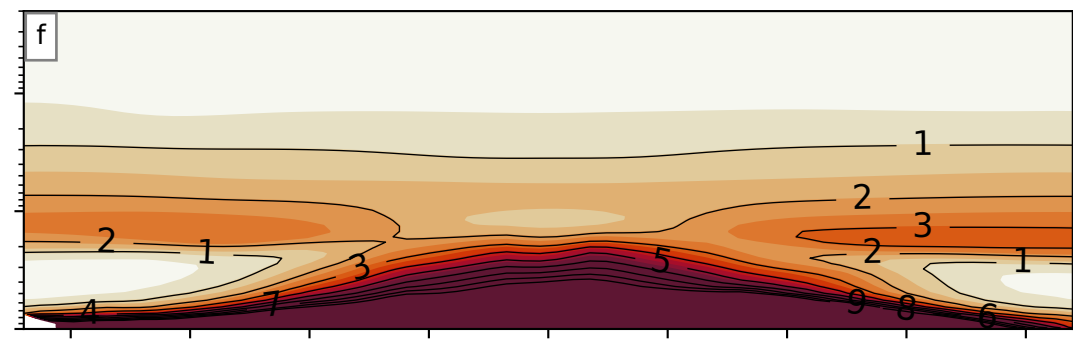
WACCM6-MAM4
