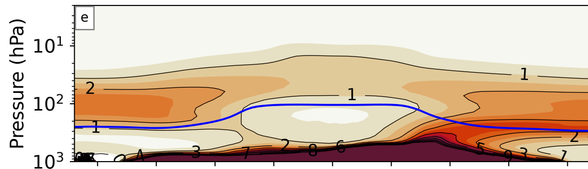
WACCM6-CARMA
