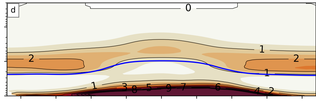
MIROC-CHASER
