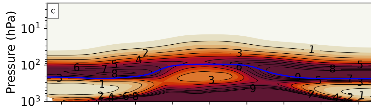
CAM5-CARMA
