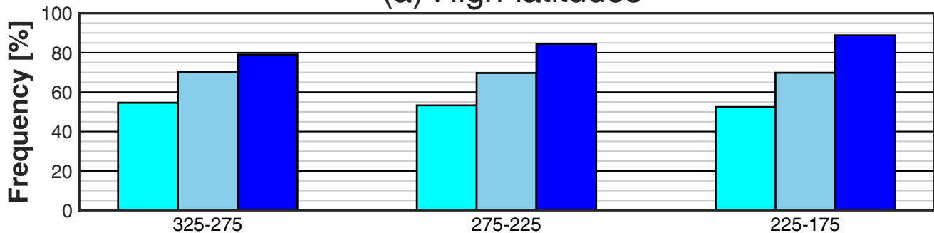
(a) High-latitudes
