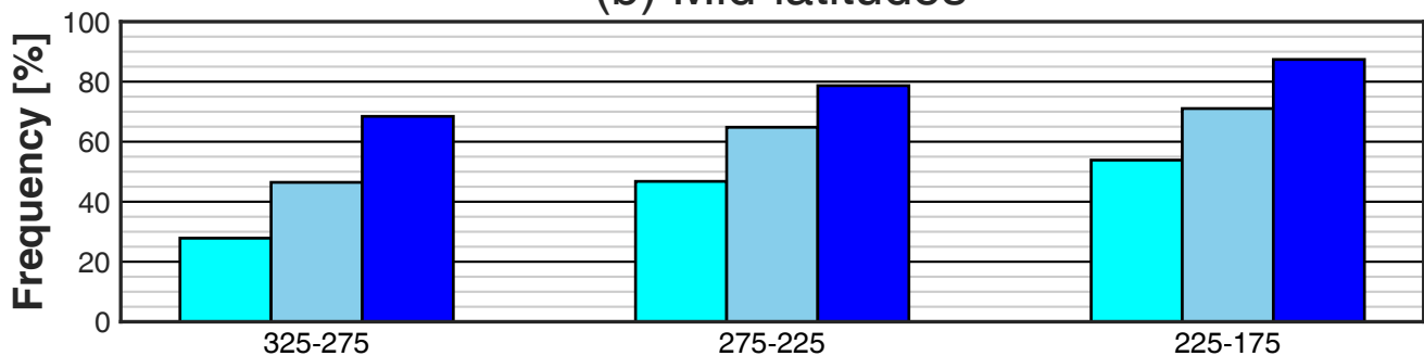
(b) Mid-latitudes
