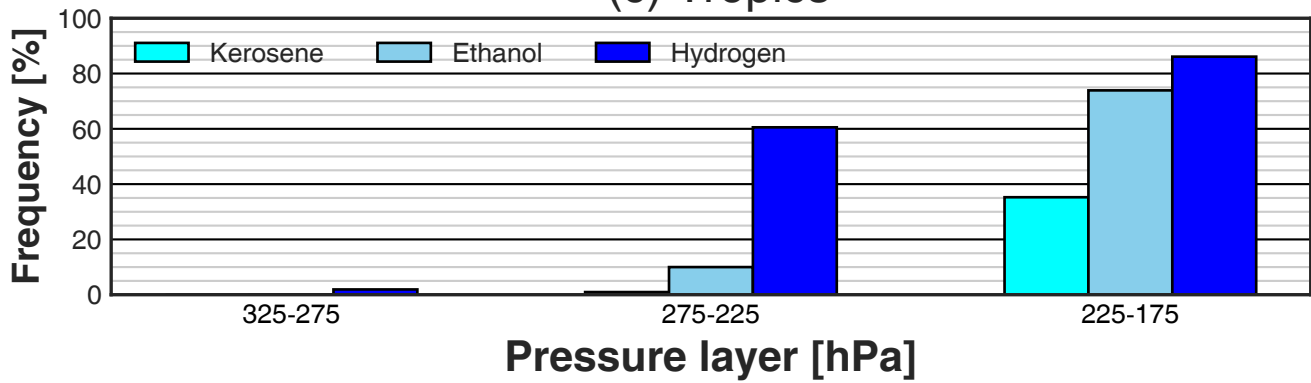
(c) Tropics
