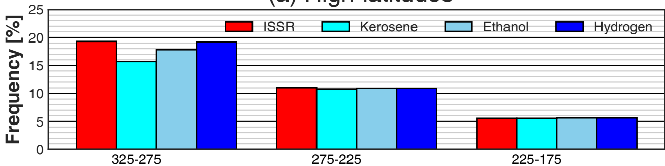
(a) High-latitudes
