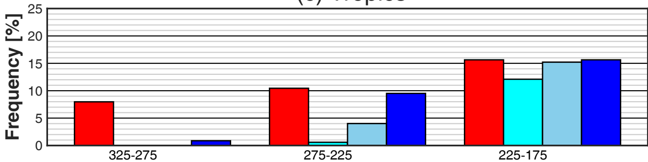
(c) Tropics
