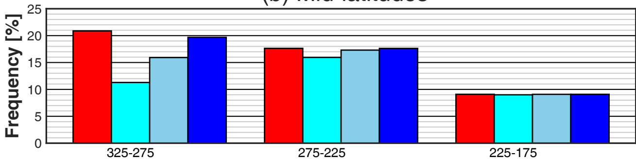
(b) Mid-latitudes
