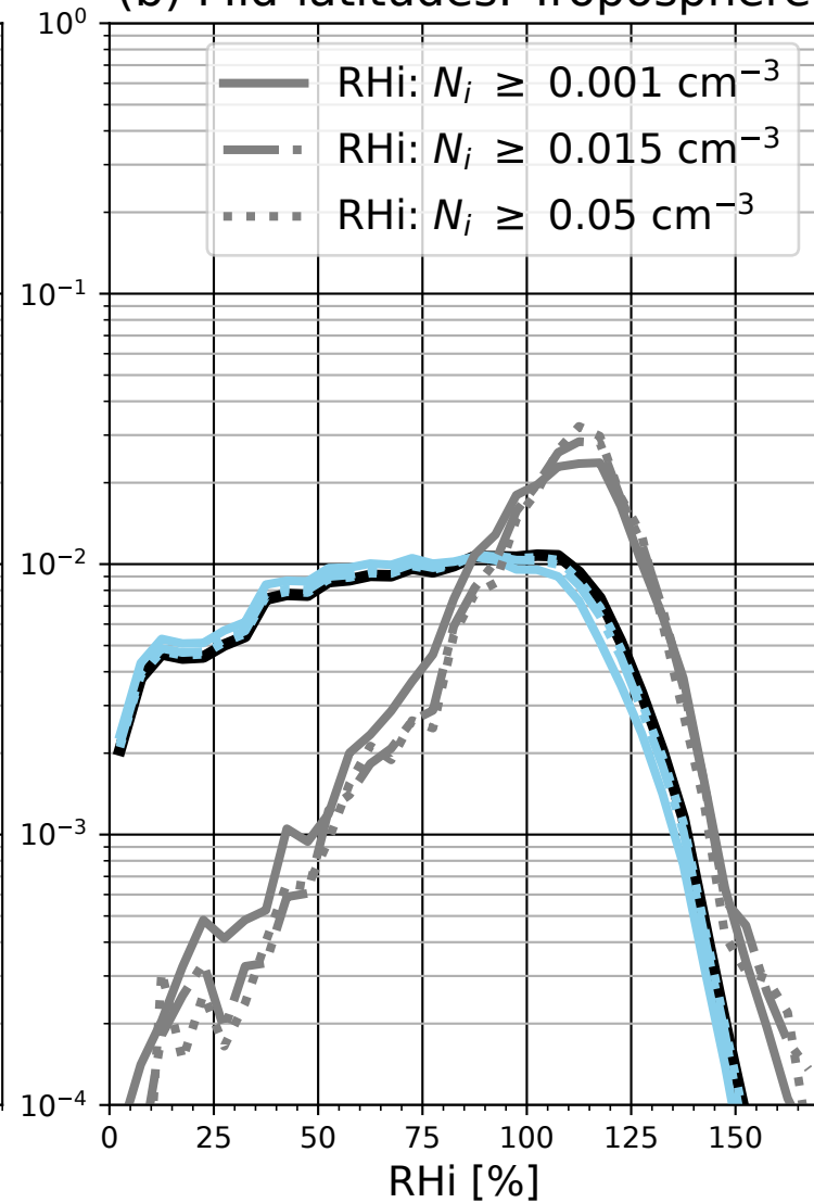
(b) Mid-latitudes: Troposphere
