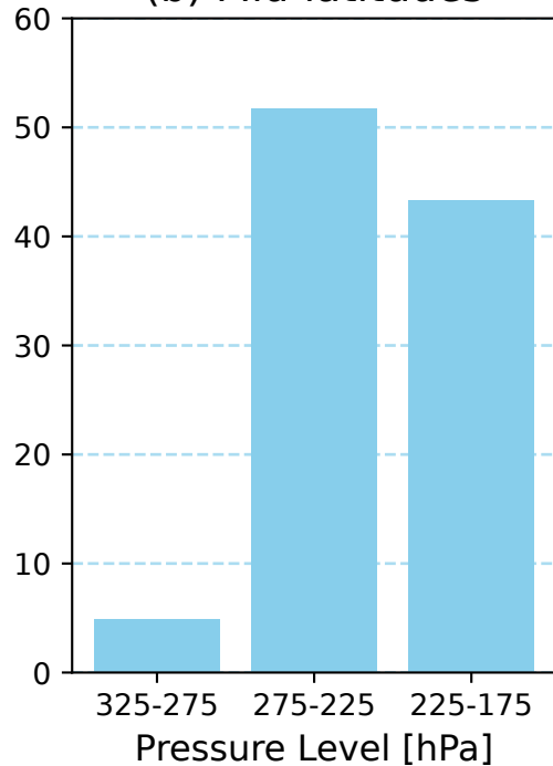
(b) Mid-latitudes
