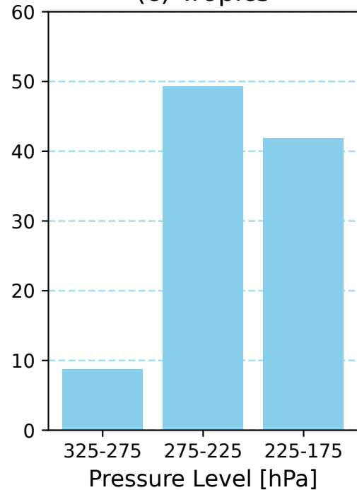
(c) Tropics
