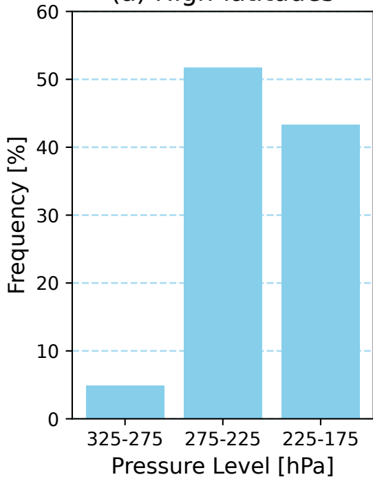
(a) High-latitudes
