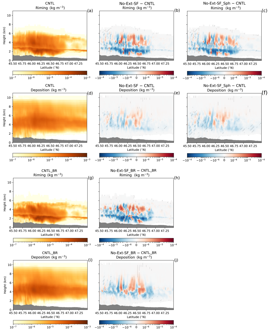
Figure S2. Cross-section of the growth of ice particles by riming (a, g) and deposition (d, i) for the CNTL and CNTL_BR simulation ensemble means, respectively. (b, c, e), are the differences between the sensitivity (No-Ext-SF and No-Ext-SF_Sph) and the CNTL simulation ensemble means. (h, j) are the differences between the No-Ext-SF_BR and CNTL_BR simulation ensemble means. The vertical (positive) and slanted (negative) black lines show where the differences are outside of the 95% confidence interval of the CNTL and CNTL_BR ensemble simulations. The cross-section is a zonal and temporal mean from 13:30 to 17:00 UTC.
