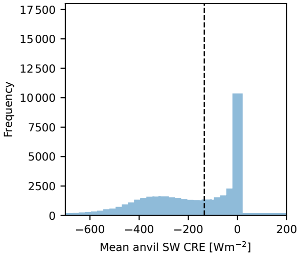
(a) SW CRE [Avg: -135.0 \pm 0.9 \text{ Wm}^{-2} ]
