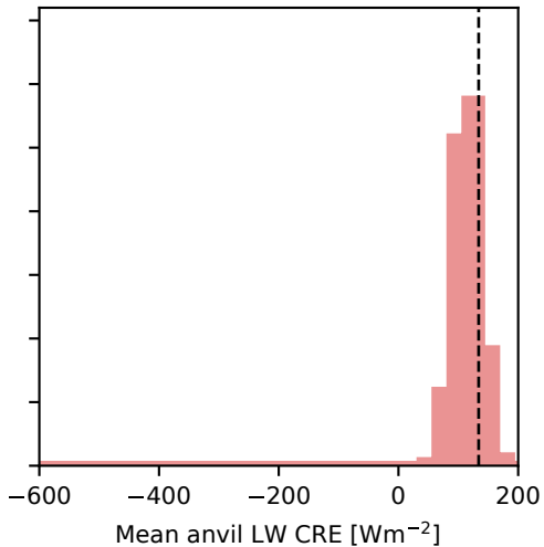
(b) LW CRE [Avg: 134.0 \pm 0.1 \text{ Wm}^{-2} ]
