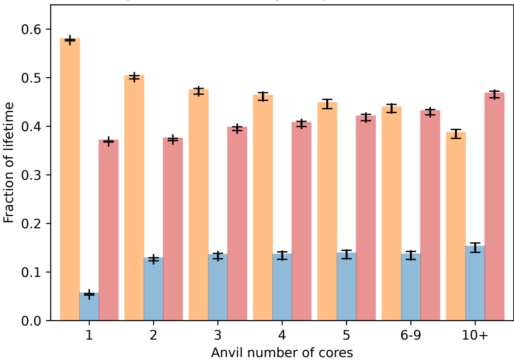
Proportional anvil lifecycle by number of cores
