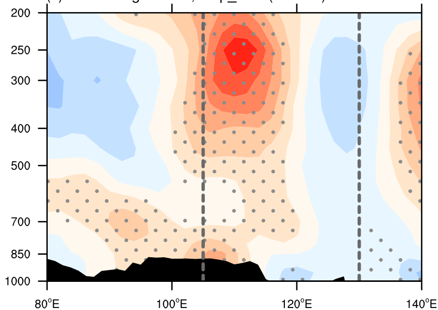
(c) Partial Reg<-IOBM,temp_adv>(38-46N)
