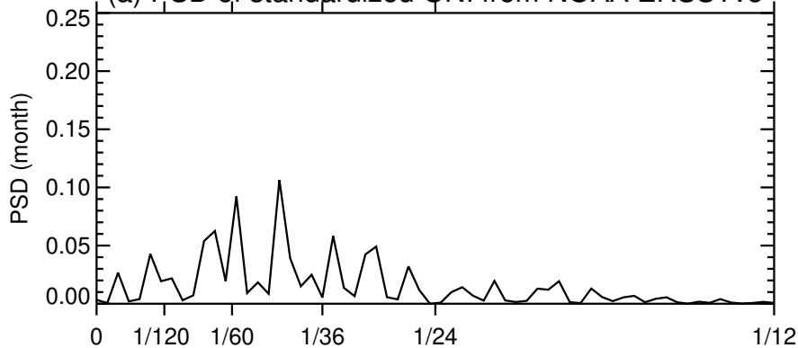
(a) PSD of standardized QNI from NOAA ERSSTv5
