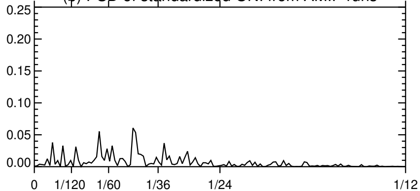
(b) PSD of standardized QNI from AMIP runs
