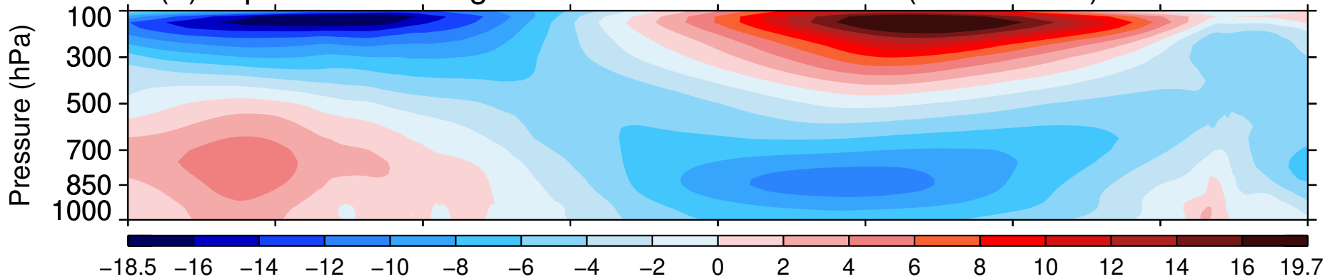
(b) Equatorial \bar{u} averaged over all El Niño months (1979–2015) from ERA5
