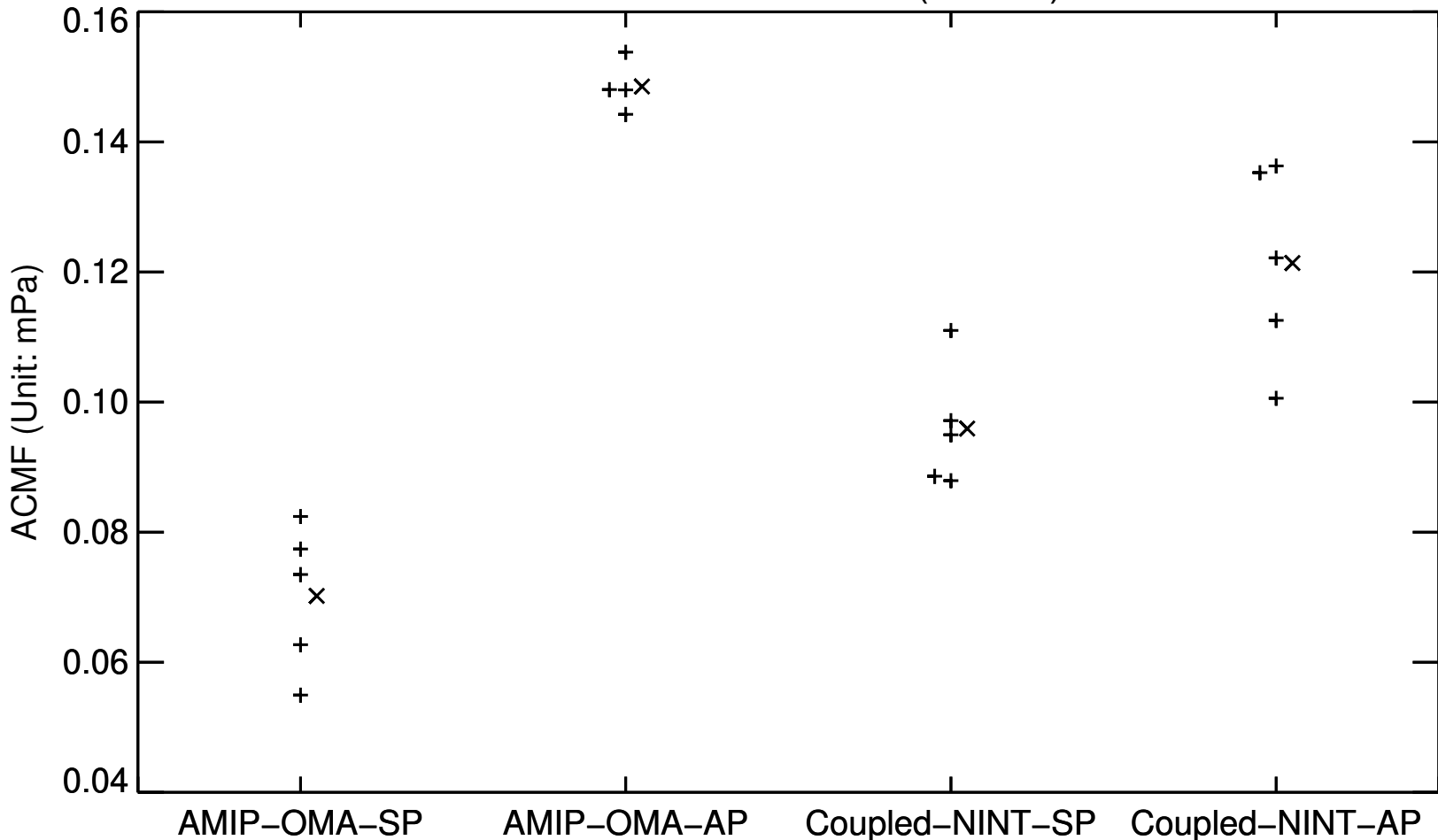
Absolute convective momentum fluxes (ACMF) at source altitude
