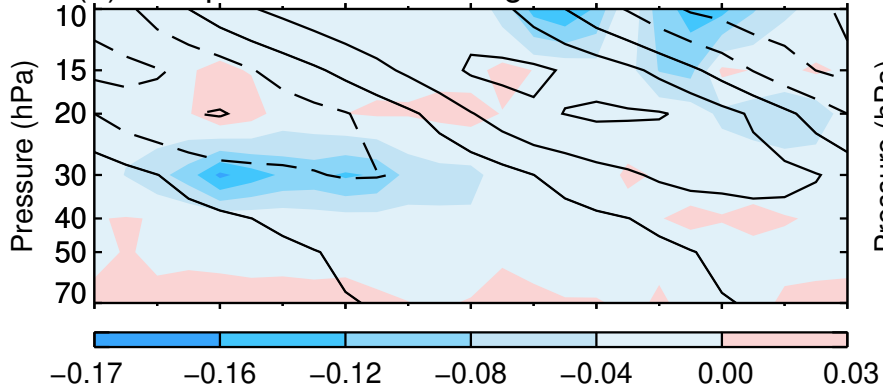
(a) Comp. diff of GW forcing between EN and LN
