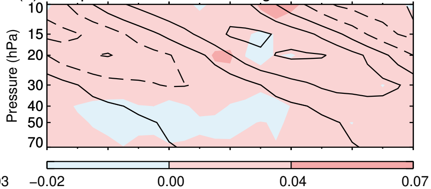
(b) Comp. diff of resolved forcing between EN and LN
