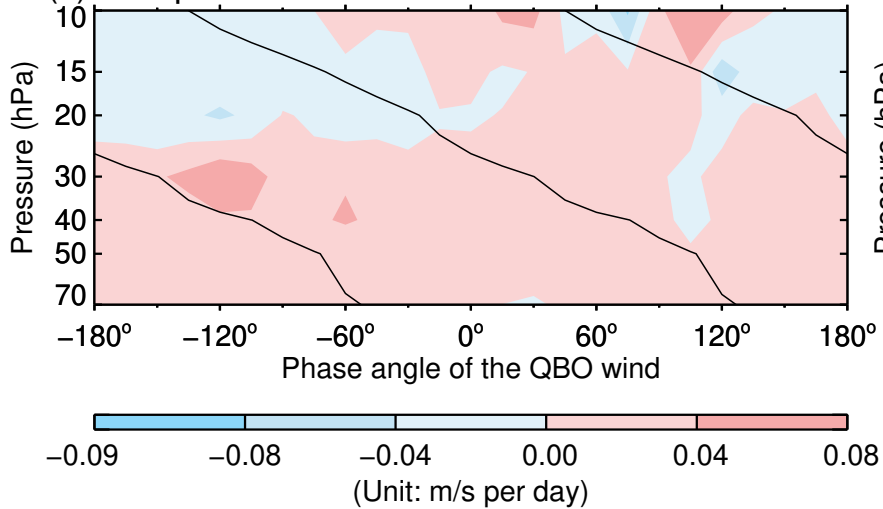
(c) Comp. diff of TEM advection between EN and LN
