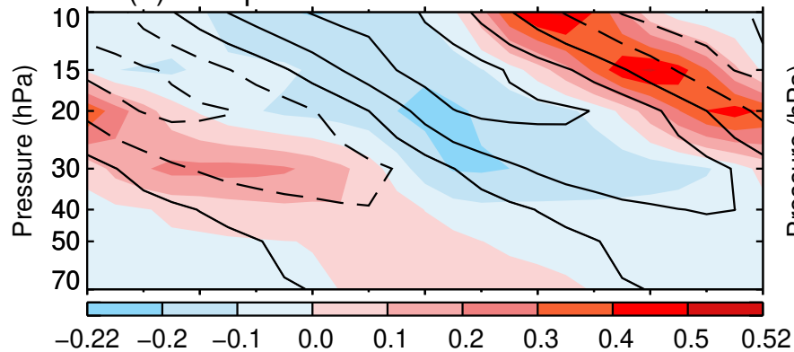
(b) Composite TEM advection for El Niño
