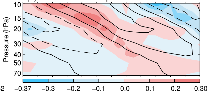
(e) Sum of three composite terms for El Niño
