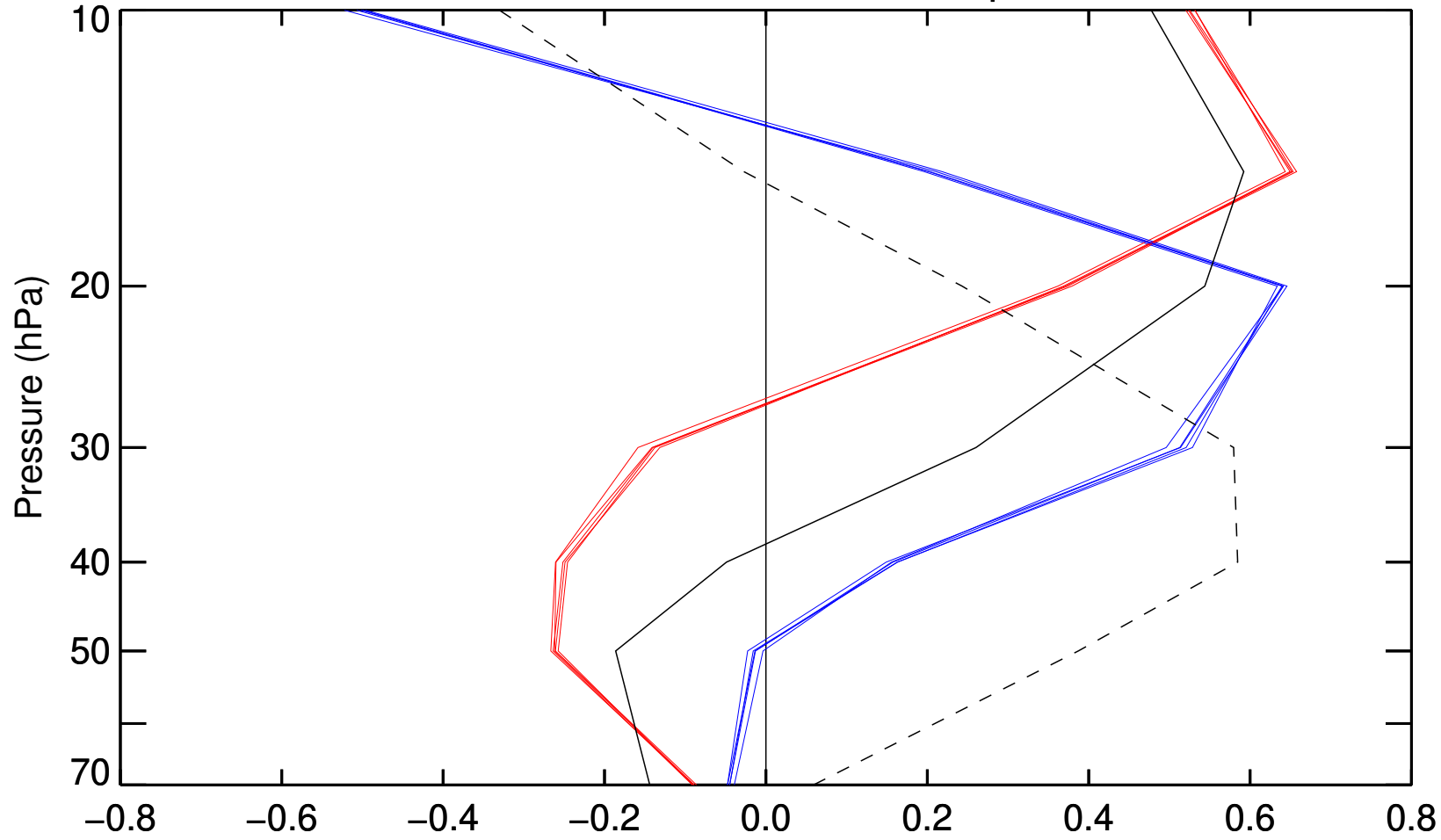
EOFs 1 and 2 from the FUB data and Coupled-NINT-AP runs
