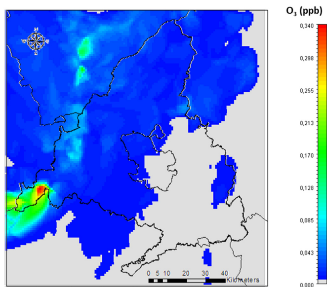
Figure S4. Maximum 1-hour attribution of stratospheric transport (ST) to ground-level O 3 .
