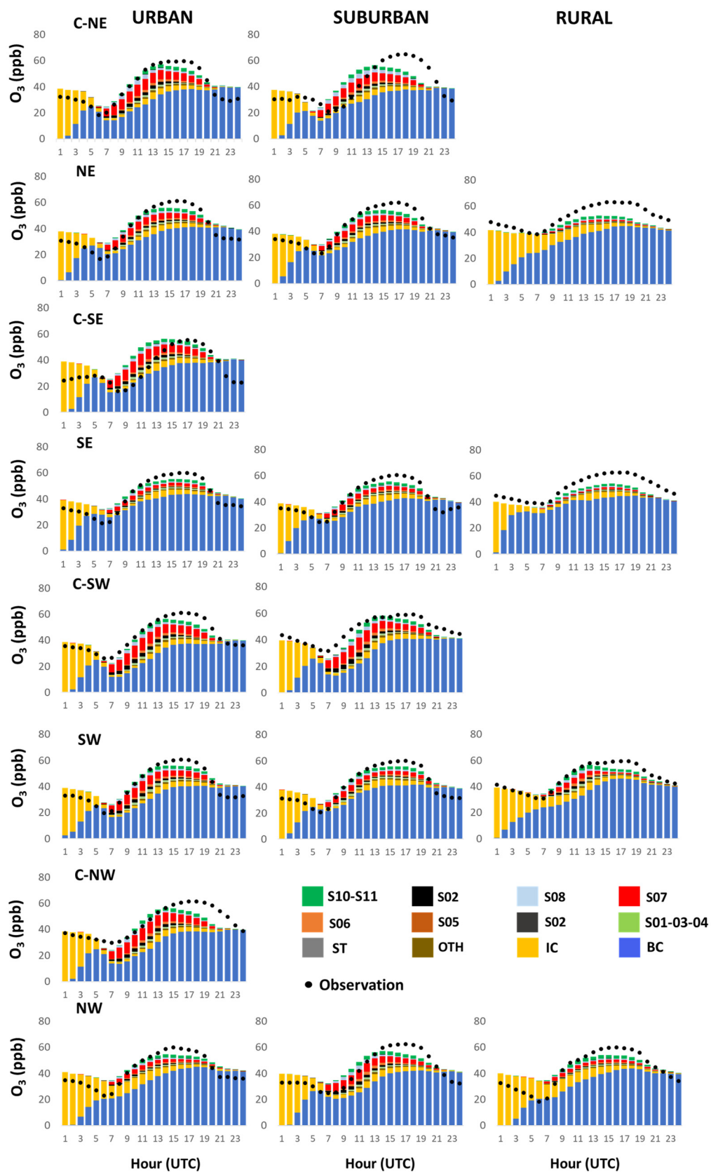
Figure S14. Hourly contribution to ground-level O_3 (ppb) for the monthly average at the location of monitoring sites by geographical quadrant.
