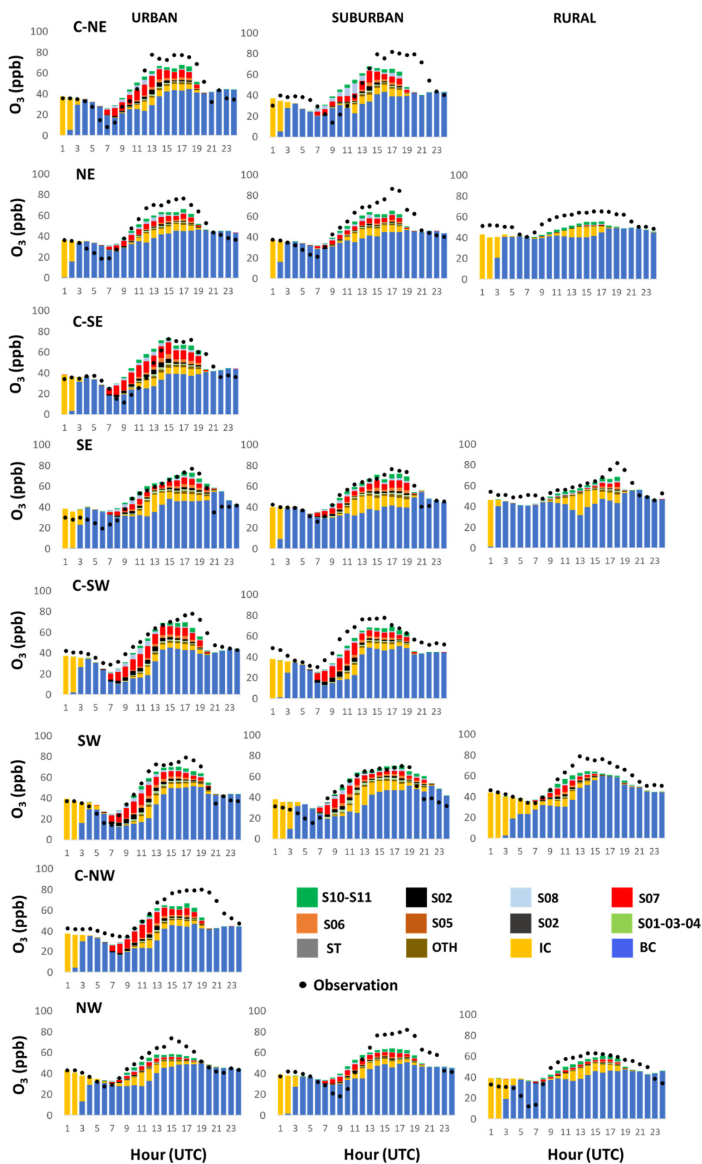
Figure S15. Hourly contribution to ground-level O 3 (ppb) for July 27 th , 2016 at the location of monitoring sites by geographical quadrant.
