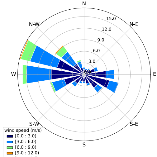
ERA5 at 100 m (Yangquan)
