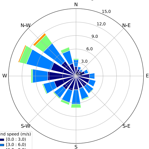
ERA5 at 100 m (Changzhi)
