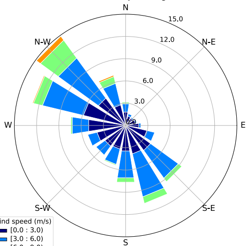
ERA5 at 100 m (Jincheng)
