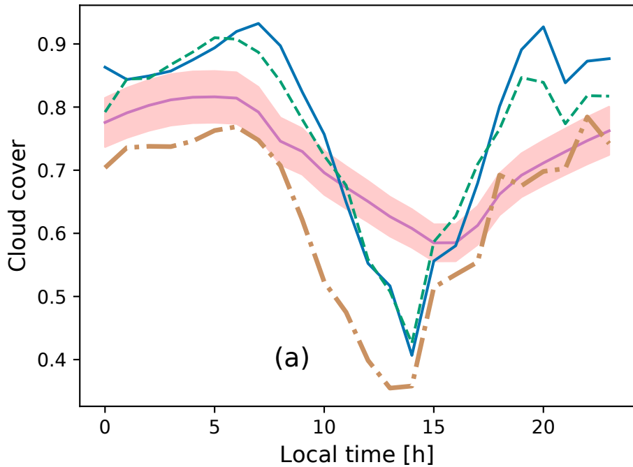
Cloud cover
