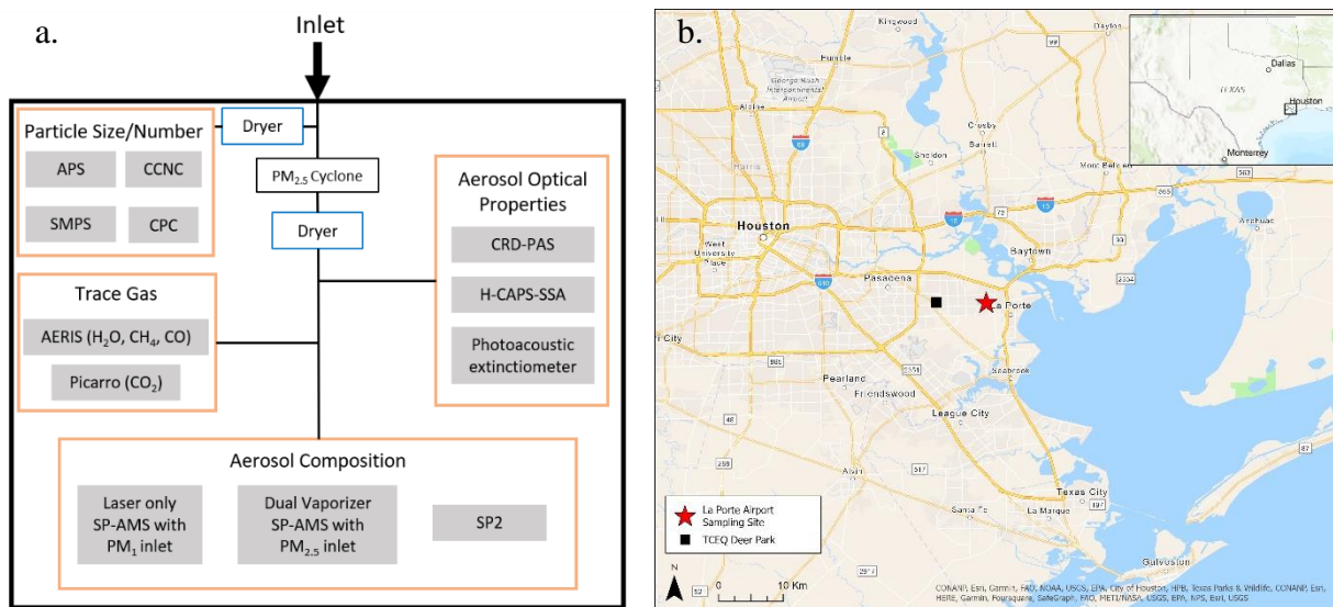
110 Figure S1: (a) Schematic of the experimental layout during the TRACER field campaign. Acronyms: APS: Aerodynamic Particle Sizer, CCNC: Cloud Condensation Nuclei Counter, SMPS: Scanning Mobility Particle Sizer, CPC: Condensation Particle Counter, CRD-PAS: Cavity Ring Down- Photoacoustic Spectrometer, H-CAPS-SSA: Humidified cavity-attenuated phase shift-single scattering albedo monitor, SP2: Single Particle Soot Photometer. (b) Map depicting the location of the La Porte sampling site (red star) in the greater Houston region.
