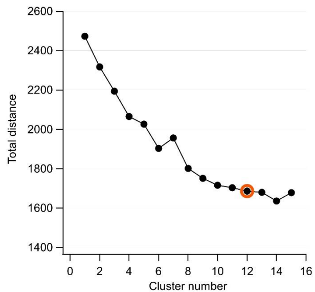
Figure S2: Total Euclidian distance between individual particles and the cluster average as a function of cluster number. The final 12-cluster solution is marked with the orange circle.
