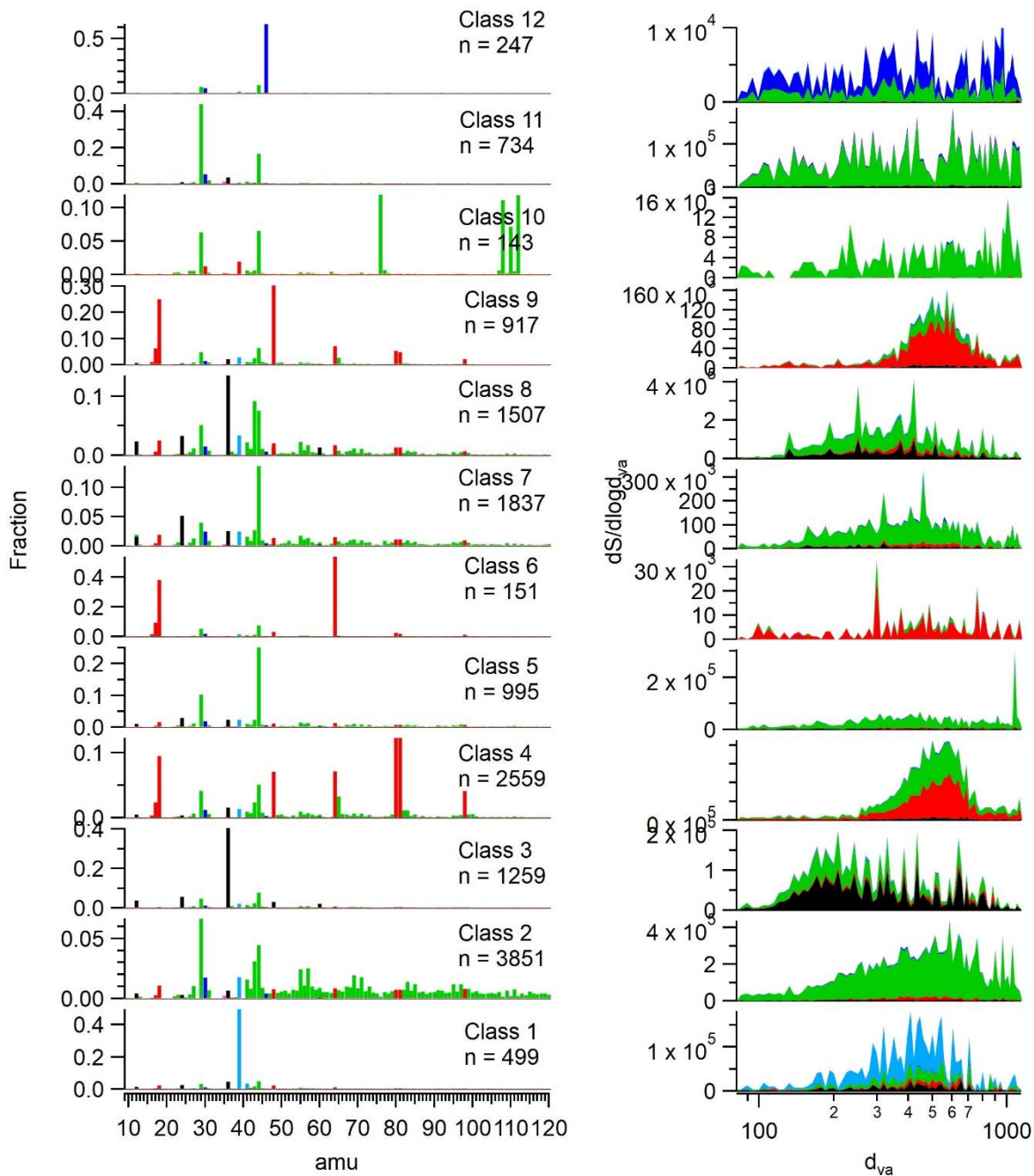
Figure S3: Average mass spectra and size distributions of particle clusters prior to merging similar clusters. Clusters 4, 6 and 9 were merged into a single sulfate cluster. Clusters 5 and 7 were merged into a single OOA cluster. Class 10 was discarded as a noise artifact.
