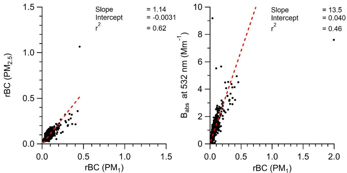
135 Figure S6: (a) Correlation between rBC measured by dual vaporizer SP-AMS equipped with PM 2.5 lens and laser-only SP-AMS. (b) Correlation between aerosol absorption at 532nm measured by photoacoustic spectroscopy and rBC measured by laser-only SP-AMS. Fit lines are orthogonal distance regressions.
