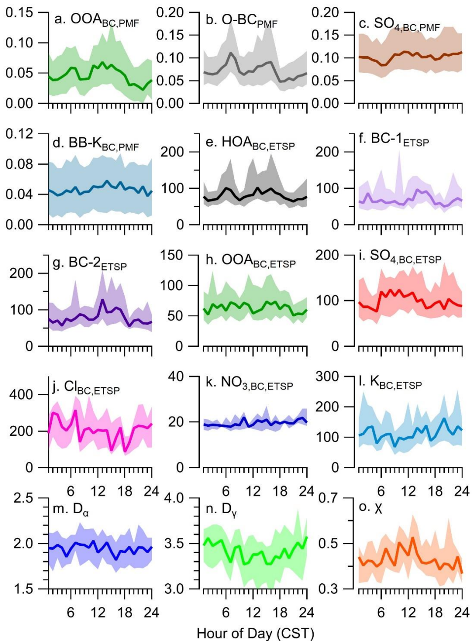
Figure S7: diurnal profiles of (a-d) PMF factors, (e-l) ETSP particle clusters, (m-o) mixing state metrics. Solid line is hourly median value and shaded area represents the interquartile range. Units for a-d are \mu\text{g m}^{-3} and e-l are ions.
