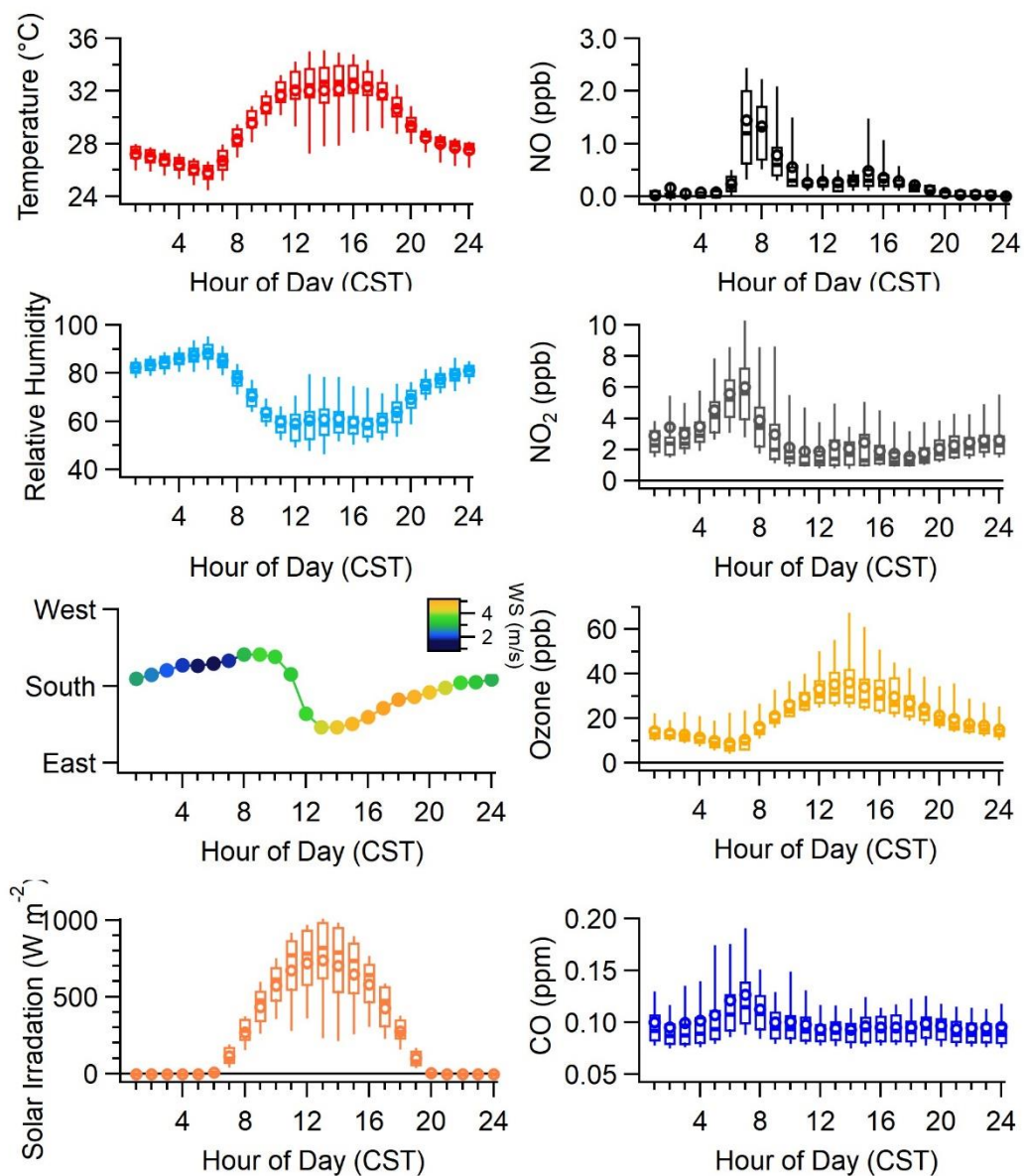
130 Figure S5: Diurnal variation in meteorological parameters and trace gas species. Solid and open symbols represent the median and mean respectively. Boxes indicate 25-75 th percentile and whiskers indicate 10-90 th percentiles.
