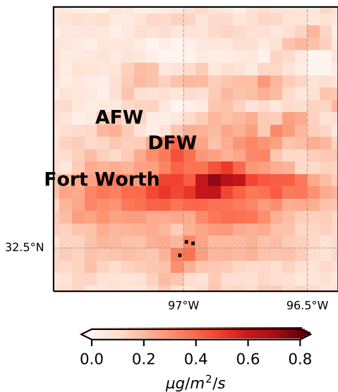
(a) derived emission E
