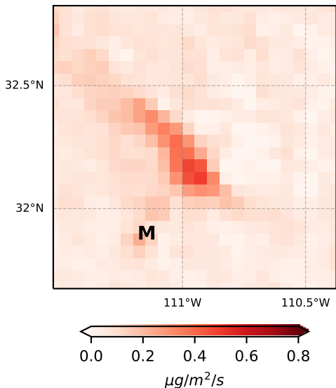
(c) derived emission E
