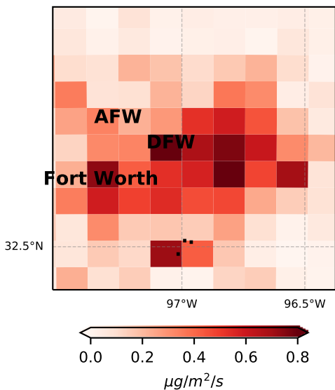
(b) NEI emission E_{NEI}
