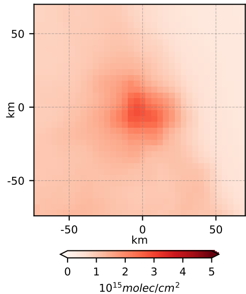
(a) \text{NO}_2 VCD
