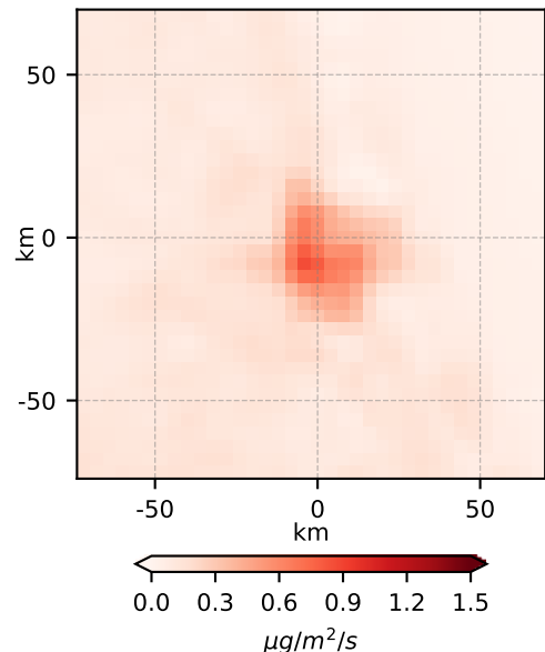
(c) derived \text{NO}_x emission E_{\text{NU-WRF}}
