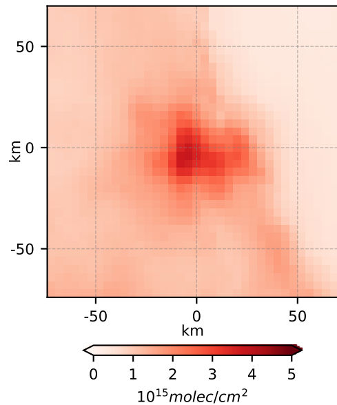
(b) \text{NO}_2 VCD under calm wind
