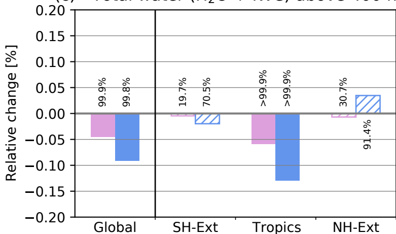
(c) - Total water (H 2 O + IWC) above 400 hPa
