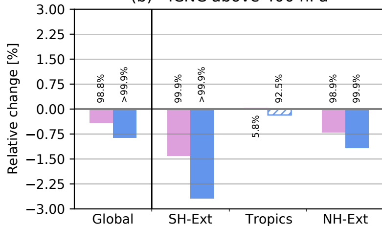
(b) - ICNC above 400 hPa
