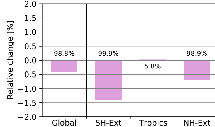
(f) - ICNC above 400 hPa
