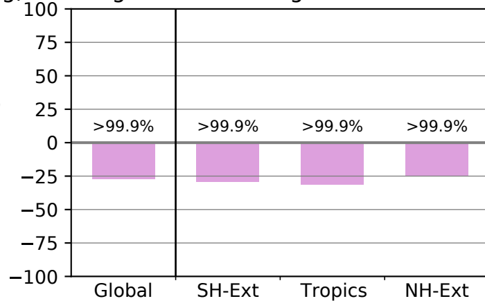
(g) - Homogeneous freezing fraction above 400 hPa
