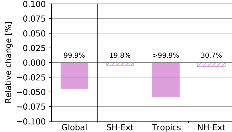
(h) - Total water (H 2 O + IWC) above 400 hPa
