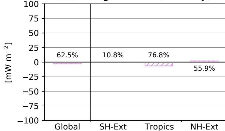
(e) - Longwave ERF (clear-sky)
