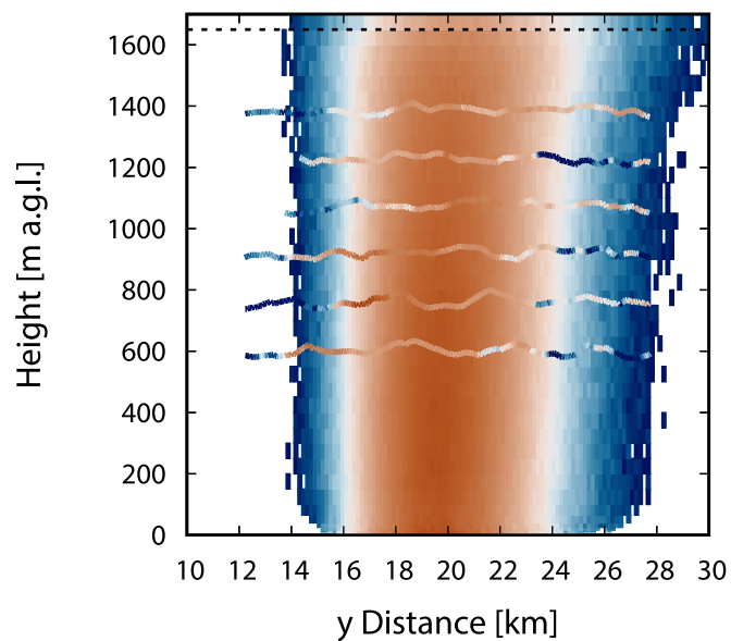
(f) ARTM2, alternating wind
