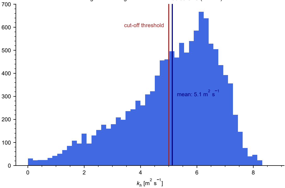
Histogram of mixing coefficients at 12:00:00 UTC (surface)
