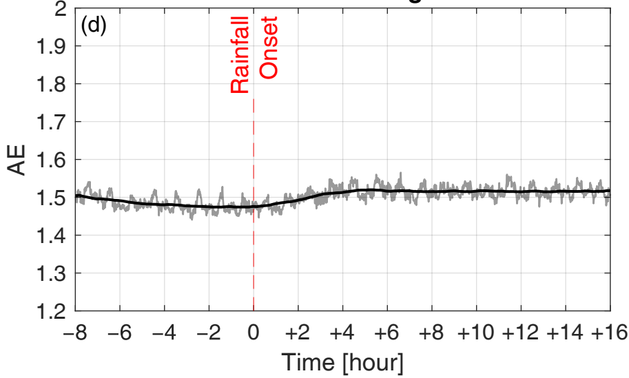
AE before and during rainfall
