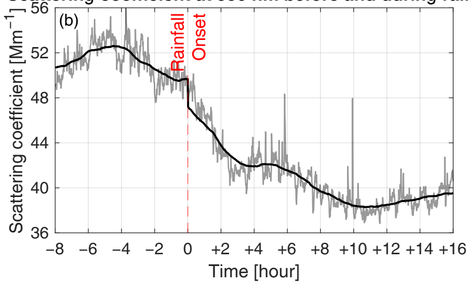
AE before and after rainfall
