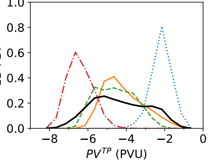
(c) DJF SH, 1D PDFs
