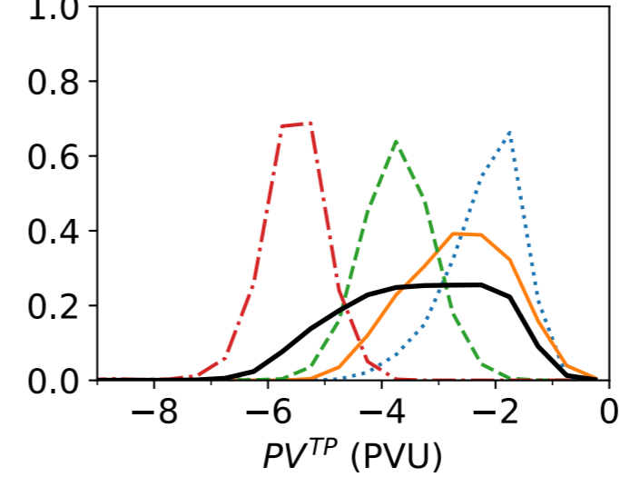
(g) JJA SH, 1D PDFs
