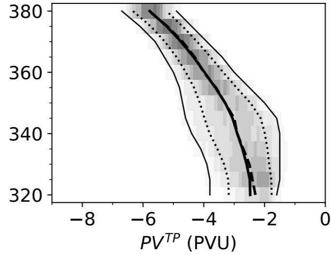
(g) JJA SH, 1D PDFs
