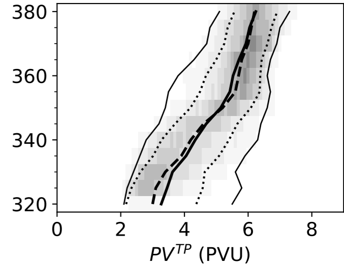
(h) JJA NH, 1D PDFs
