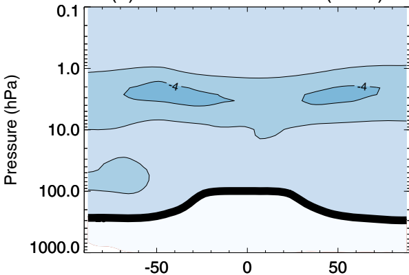
(c) Ozone % diff (2020)
