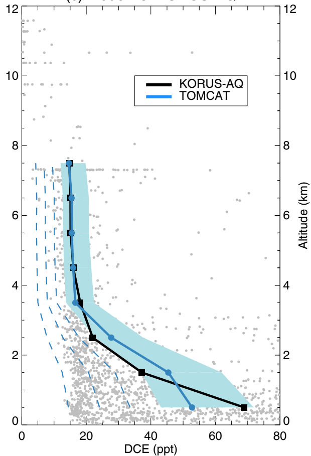
(c) Model vs. KORUS-AQ
