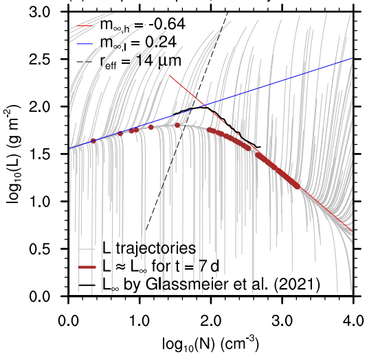
(a) L-N phase space, full N dynamics
