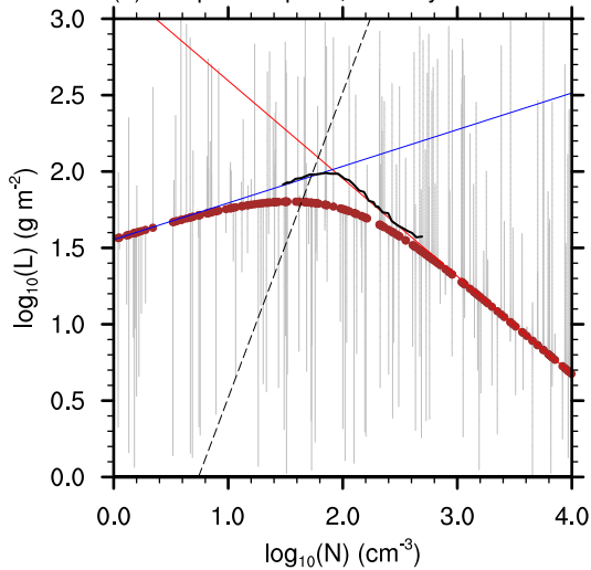
(b) L-N phase space, no N dynamics
