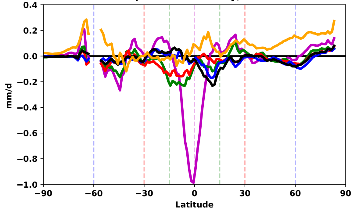
(b) \Delta Precipitation (land only, 2050-2069)
