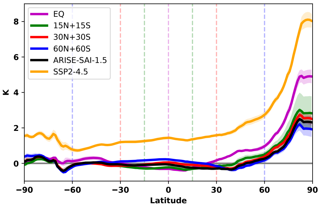
(c) \Delta Ts (2050-2069)
