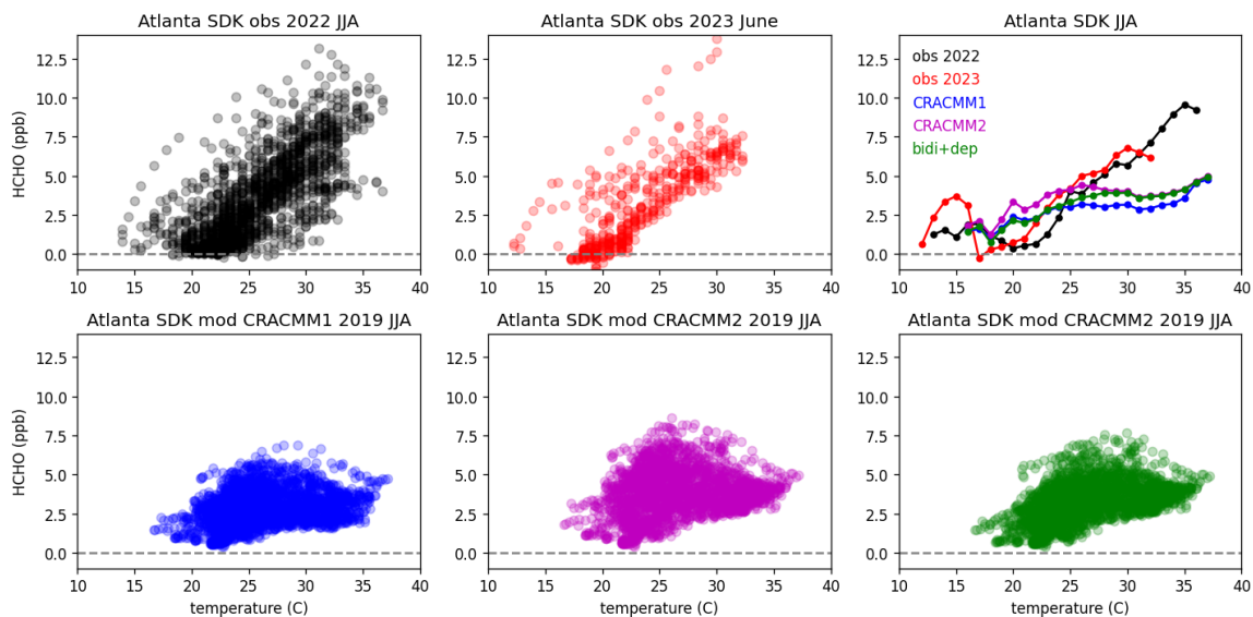
330 Figure S21. Hourly HCHO concentration by temperature at the Atlanta, GA South DeKalb (SDK) sampling location during summer. All available hourly data points are provided for the 2022 and 2023 observations and for the CRACMM1, CRACMM2, and bidi+dep CMAQ simulations. The upper right panel shows the median temperature in 1 degree C temperature bins for each set of observations and modeled concentrations.
