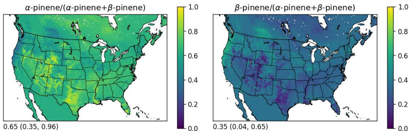
185 Figure S6. Ratio of \alpha -pinene and \beta -pinene to total pinenes based on the annual sum of biogenic emissions from BEIS. The values for \alpha -pinene and \beta -pinene include additional monoterpene emissions from BEIS that would map to these species. Monoterpenes mapped to \beta -pinene are those that have one double bond which is a terminal double bond and include \beta -pinene, camphene, and sabinene. Monoterpenes mapped to \alpha -pinene are all other monoterpenes with one double bond that is not terminal and include \alpha -pinene, \delta -3-carene, and \alpha -thujene. The annotations below each panel show the mean (min, max) over land grid cells.
