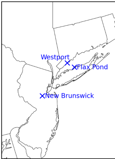
320 Figure S19. Map of sampling locations listed in Table S4. The two maps in the bottom row show a zoomed in view of the northeastern (NE) US sites and the Atlanta sites. On the map for the Atlanta sites, major roadways are displayed to provide additional geographic context.
