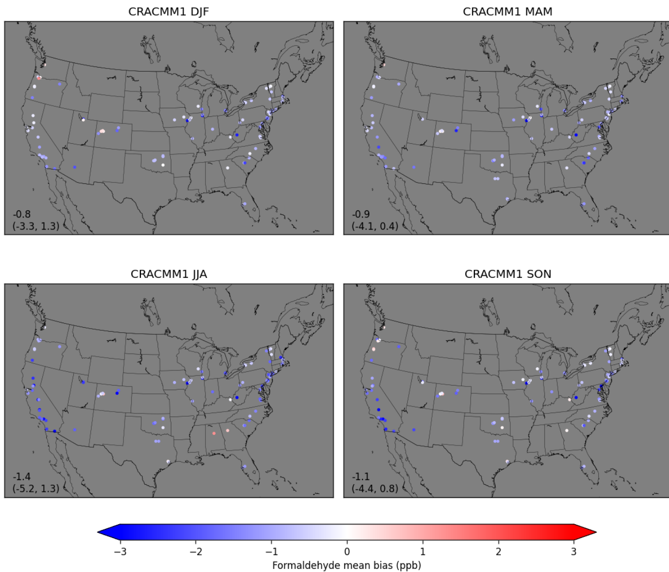
300 Figure S15. Seasonal average bias in daily average HCHO with CRACMM1 compared to observed HCHO from AQS sites. Annotations in the lower left of each panel show the mean (min, max) of seasonal average biases over all sites.
