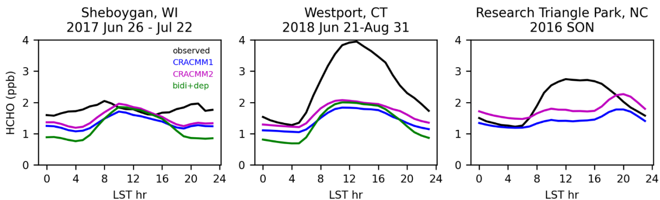
Figure S22. Diurnal profiles of observations in several years at several sites compared to CMAQ simulations in 2019 using CRACMM1, CRACMM2, and CRACMM2 with updated HCHO bidirectional flux and deposition (bidi+dep). The bidi+dep results are not shown for the Research Triangle Park, NC, site since this was a sensitivity simulation conducted for summer only. Sampling locations and dates are provided above each panel.
