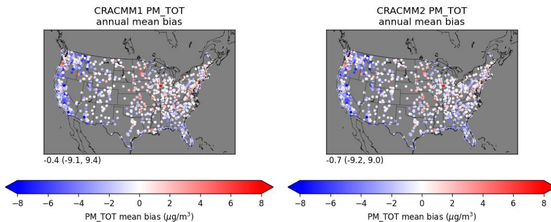
Figure S33. Annual mean bias in daily average PM 2.5 for 2019 at AQS monitoring sites for CRACMM1 (left) and CRACMM2 (right). The annotations in the lower left show the mean (min, max) site average biases.
