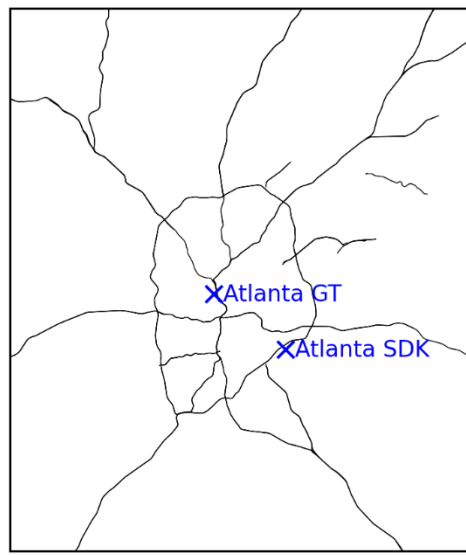
320 Figure S19. Map of sampling locations listed in Table S4. The two maps in the bottom row show a zoomed in view of the northeastern (NE) US sites and the Atlanta sites. On the map for the Atlanta sites, major roadways are displayed to provide additional geographic context.
