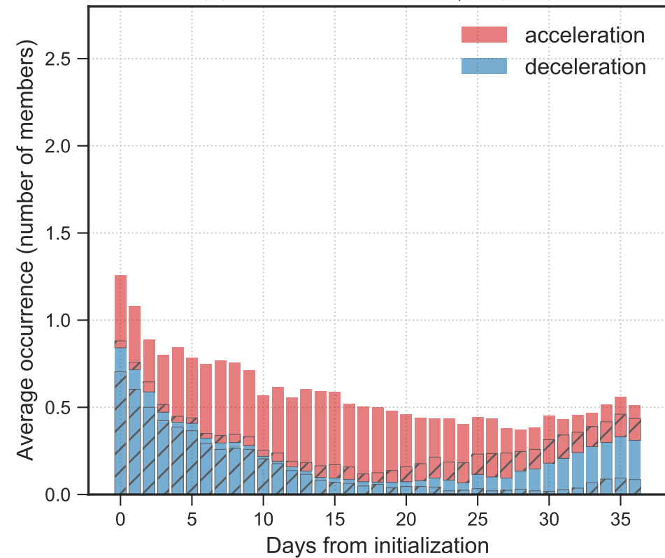
(c) Small spread in U_{10,60} (328)
