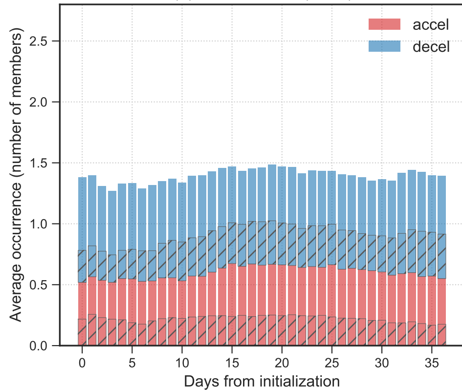
(a) All hindcasts (1311)
