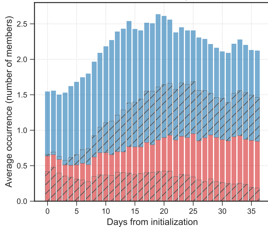
(b) Large spread in U_{10,60} (328)
